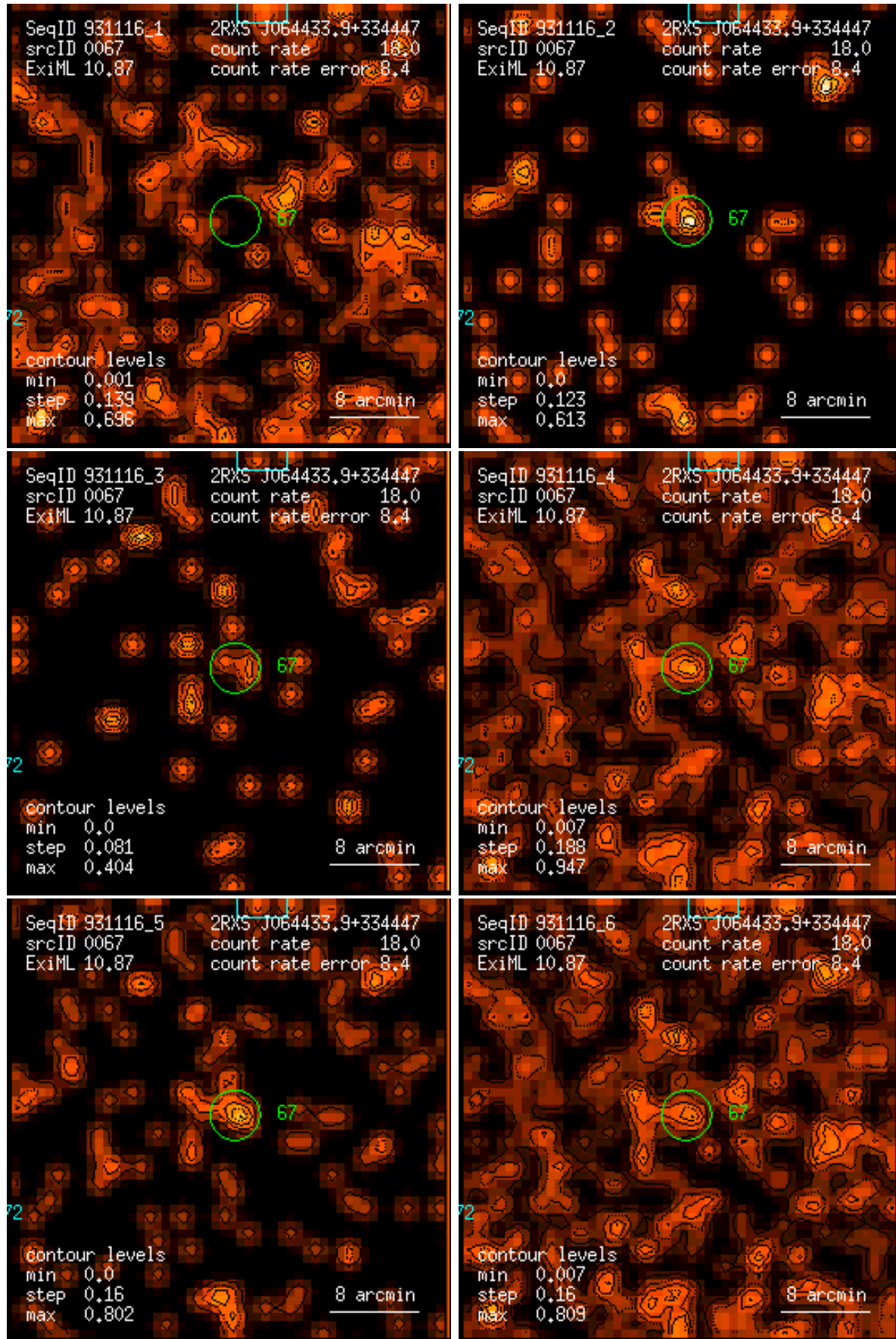
Figure 67: RASS 931116: detection 0067: band rate images, Gaussian filter: (1) PSPC channels 11 – 41, (2) 52 – 90, (3) 91 – 201, (4) 11 – 235, (5) 52 – 201, (6) 11 – 201. Broad band rates in counts/ks. Band rate contour levels in counts/ks/arcmin 2 .
