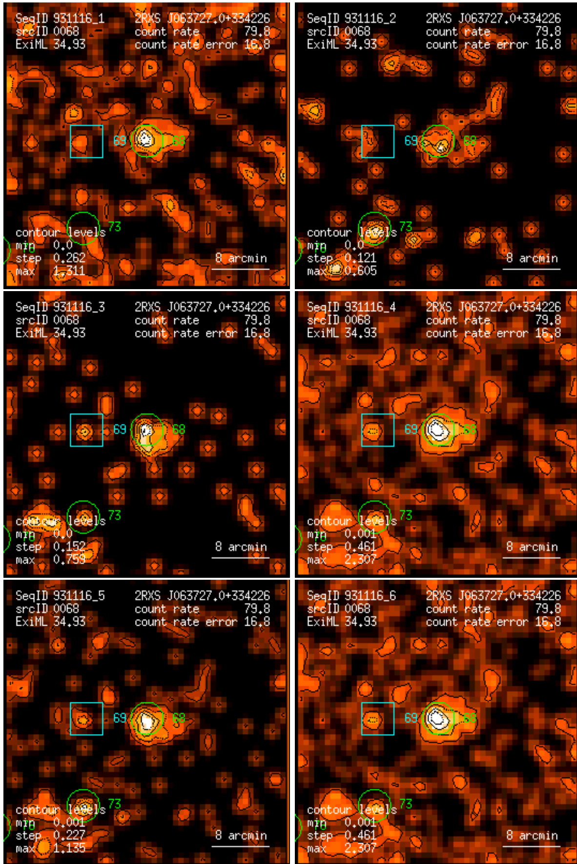
Figure 68: RASS 931116: detection 0068: band rate images, Gaussian filter: (1) PSPC channels 11 – 41, (2) 52 – 90, (3) 91 – 201, (4) 11 – 235, (5) 52 – 201, (6) 11 – 201. Broad band rates in counts/ks. Band rate contour levels in counts/ks/arcmin 2 .
