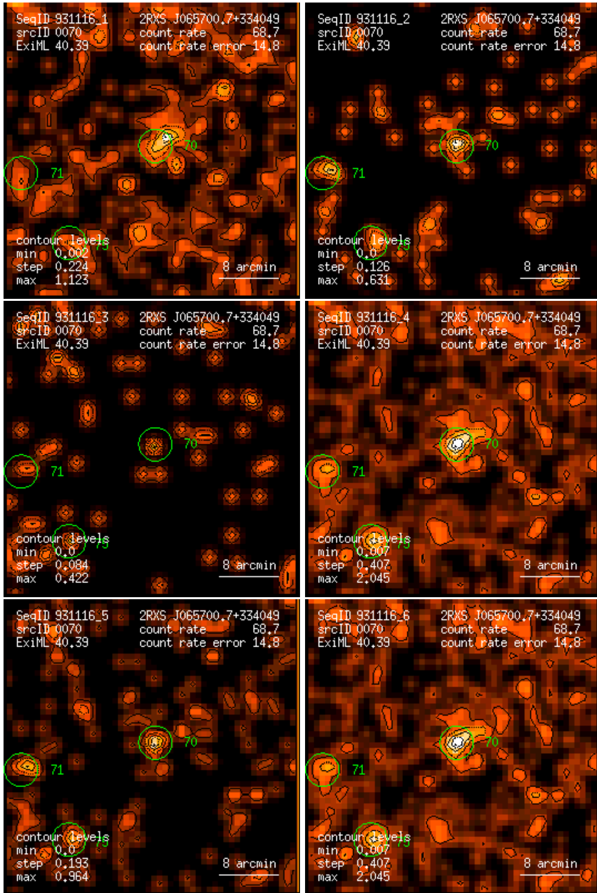
Figure 70: RASS 931116: detection 0070: band rate images, Gaussian filter: (1) PSPC channels 11 – 41, (2) 52 – 90, (3) 91 – 201, (4) 11 – 235, (5) 52 – 201, (6) 11 – 201. Broad band rates in counts/ks. Band rate contour levels in counts/ks/arcmin 2 .
