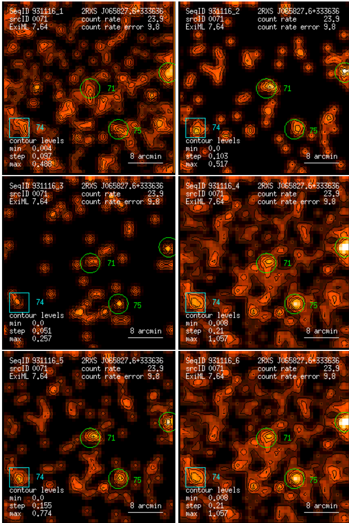
Figure 71: RASS 931116: detection 0071: band rate images, Gaussian filter: (1) PSPC channels 11 – 41, (2) 52 – 90, (3) 91 – 201, (4) 11 – 235, (5) 52 – 201, (6) 11 – 201. Broad band rates in counts/ks. Band rate contour levels in counts/ks/arcmin 2 .
