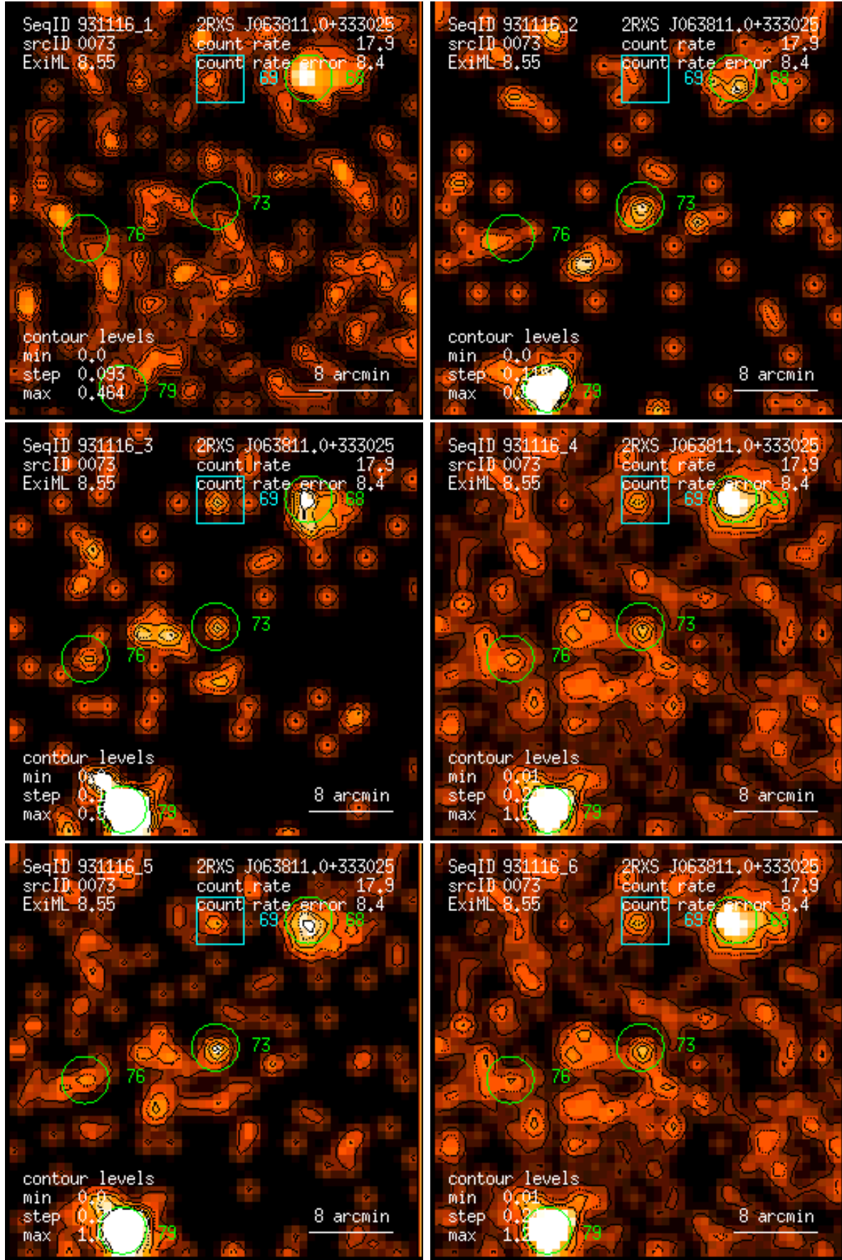
Figure 73: RASS 931116: detection 0073: band rate images, Gaussian filter: (1) PSPC channels 11 – 41, (2) 52 – 90, (3) 91 – 201, (4) 11 – 235, (5) 52 – 201, (6) 11 – 201. Broad band rates in counts/ks. Band rate contour levels in counts/ks/arcmin 2 .
