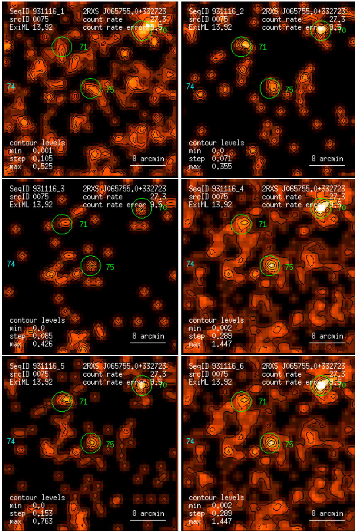
Figure 75: RASS 931116: detection 0075: band rate images, Gaussian filter: (1) PSPC channels 11 – 41, (2) 52 – 90, (3) 91 – 201, (4) 11 – 235, (5) 52 – 201, (6) 11 – 201. Broad band rates in counts/ks. Band rate contour levels in counts/ks/arcmin 2 .
