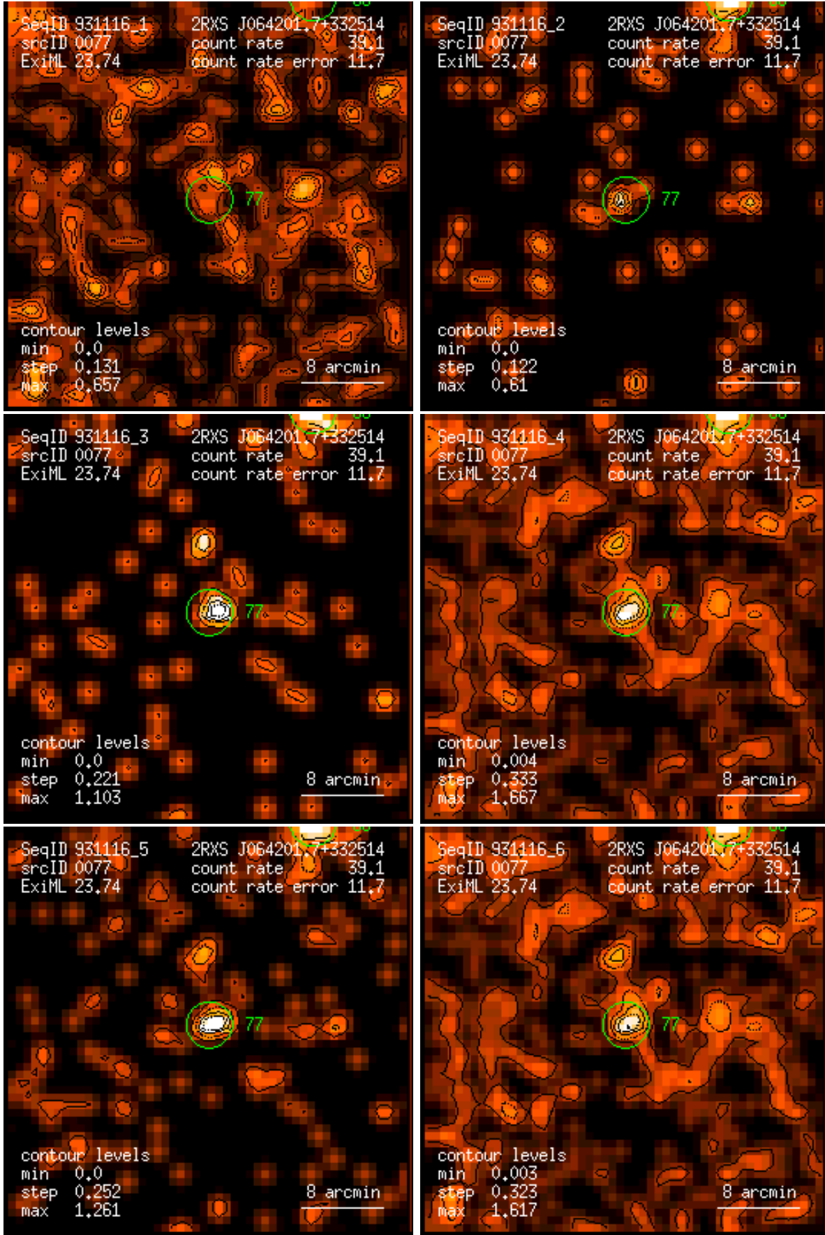
Figure 77: RASS 931116: detection 0077: band rate images, Gaussian filter: (1) PSPC channels 11 – 41, (2) 52 – 90, (3) 91 – 201, (4) 11 – 235, (5) 52 – 201, (6) 11 – 201. Broad band rates in counts/ks. Band rate contour levels in counts/ks/arcmin 2 .
