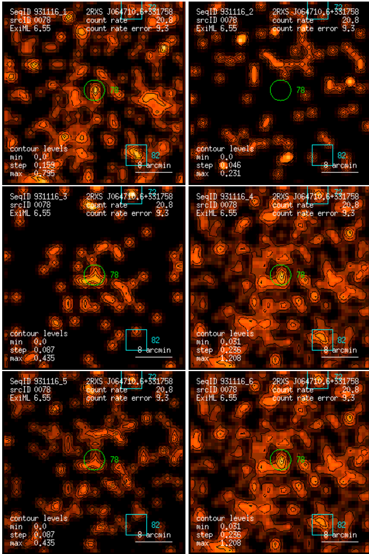
Figure 78: RASS 931116: detection 0078: band rate images, Gaussian filter: (1) PSPC channels 11 – 41, (2) 52 – 90, (3) 91 – 201, (4) 11 – 235, (5) 52 – 201, (6) 11 – 201. Broad band rates in counts/ks. Band rate contour levels in counts/ks/arcmin 2 .
