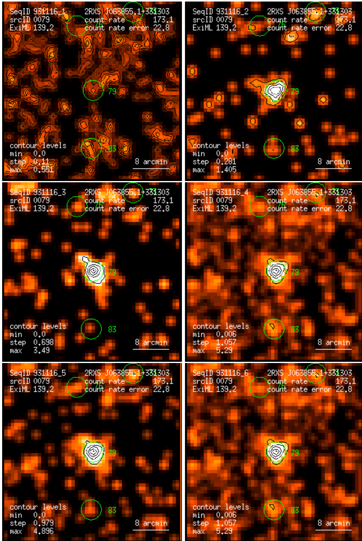
Figure 79: RASS 931116: detection 0079: band rate images, Gaussian filter: (1) PSPC channels 11 – 41, (2) 52 – 90, (3) 91 – 201, (4) 11 – 235, (5) 52 – 201, (6) 11 – 201. Broad band rates in counts/ks. Band rate contour levels in counts/ks/arcmin 2 .
