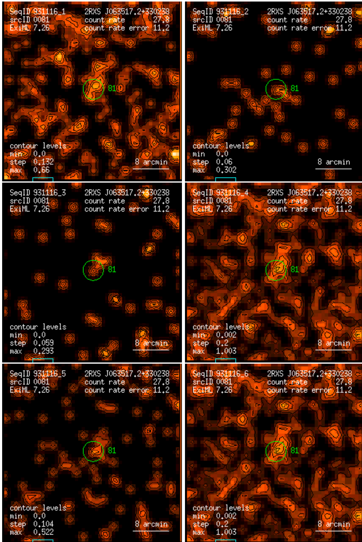
Figure 81: RASS 931116: detection 0081: band rate images, Gaussian filter: (1) PSPC channels 11 – 41, (2) 52 – 90, (3) 91 – 201, (4) 11 – 235, (5) 52 – 201, (6) 11 – 201. Broad band rates in counts/ks. Band rate contour levels in counts/ks/arcmin 2 .
