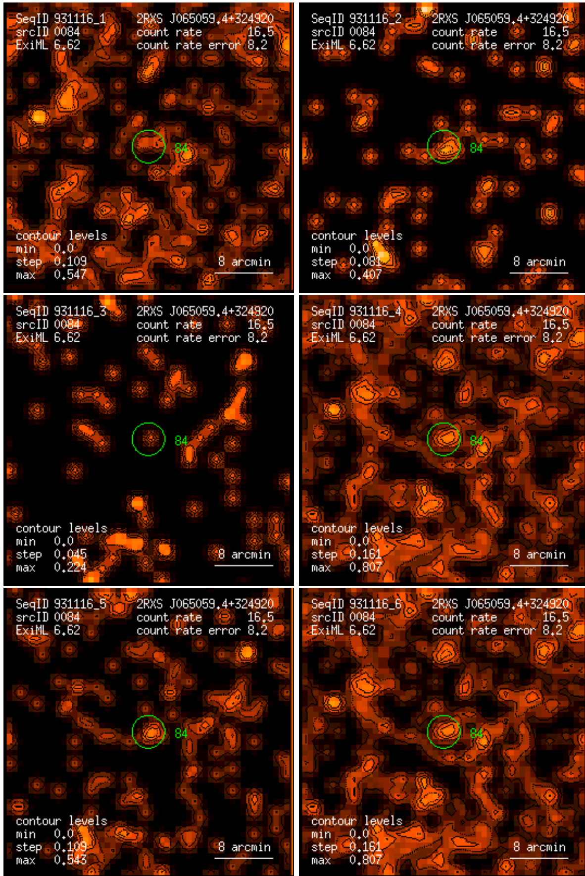
Figure 84: RASS 931116: detection 0084: band rate images, Gaussian filter: (1) PSPC channels 11 – 41, (2) 52 – 90, (3) 91 – 201, (4) 11 – 235, (5) 52 – 201, (6) 11 – 201. Broad band rates in counts/ks. Band rate contour levels in counts/ks/arcmin 2 .
