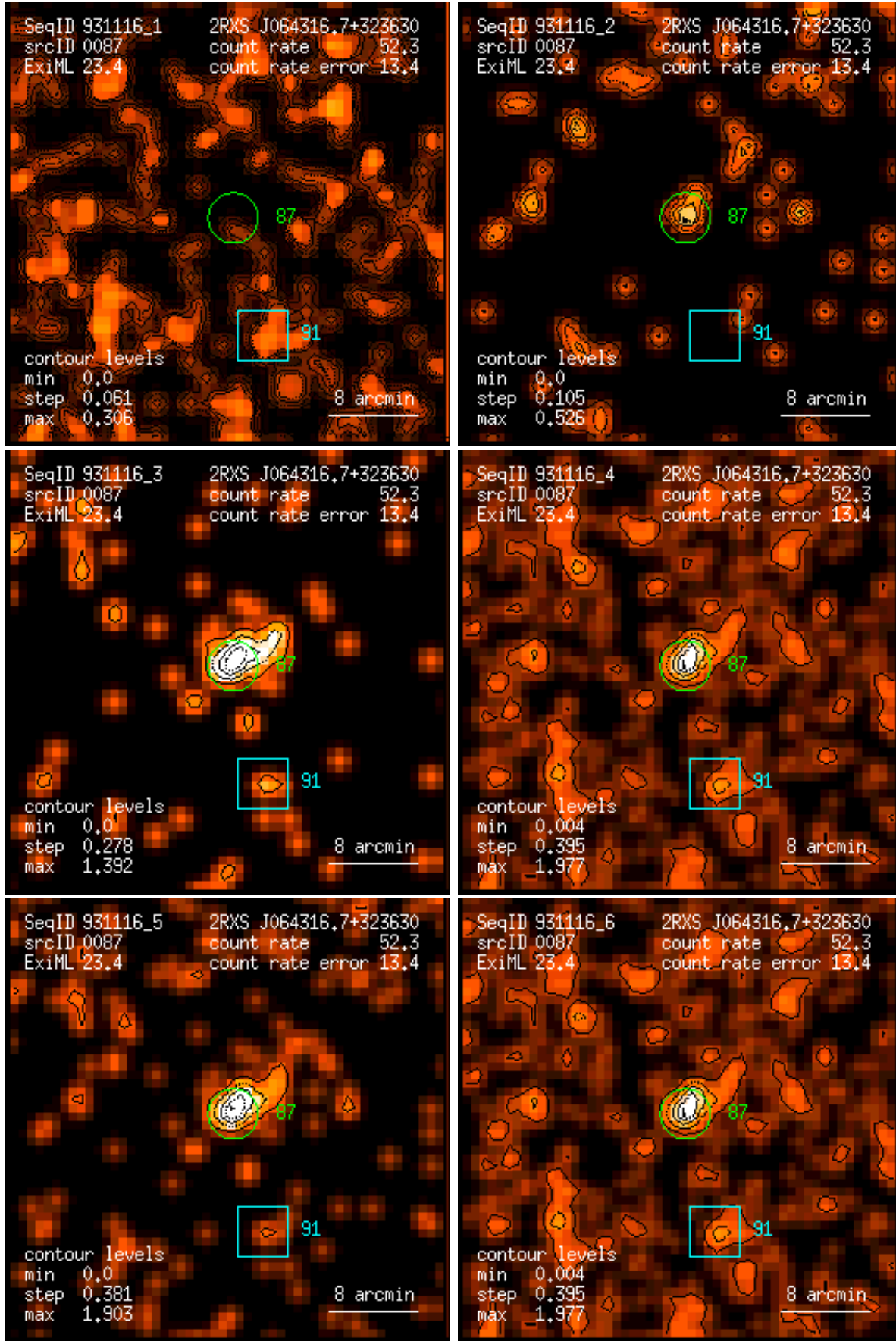
Figure 87: RASS 931116: detection 0087: band rate images, Gaussian filter: (1) PSPC channels 11 – 41, (2) 52 – 90, (3) 91 – 201, (4) 11 – 235, (5) 52 – 201, (6) 11 – 201. Broad band rates in counts/ks. Band rate contour levels in counts/ks/arcmin 2 .
