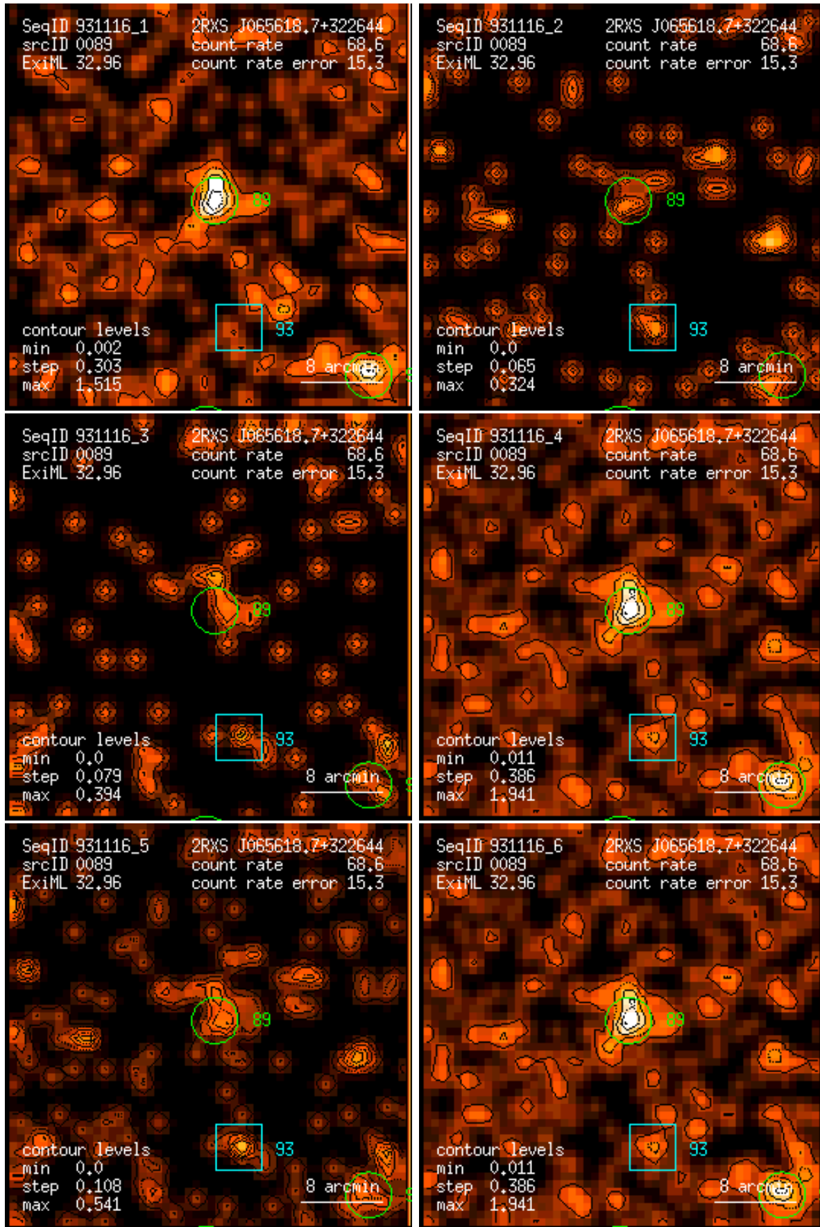
Figure 89: RASS 931116: detection 0089: band rate images, Gaussian filter: (1) PSPC channels 11 – 41, (2) 52 – 90, (3) 91 – 201, (4) 11 – 235, (5) 52 – 201, (6) 11 – 201. Broad band rates in counts/ks. Band rate contour levels in counts/ks/arcmin 2 .
