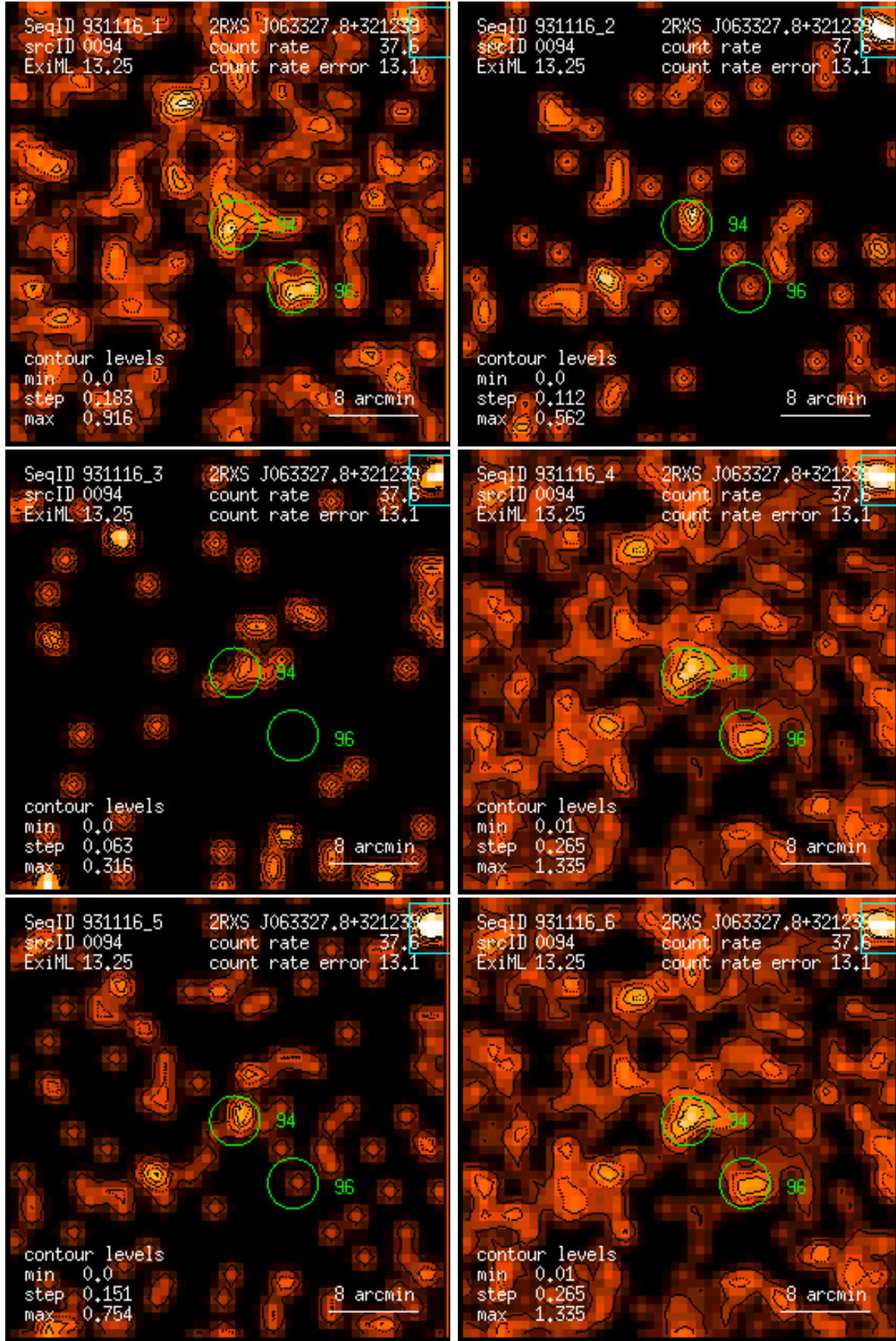
Figure 94: RASS 931116: detection 0094: band rate images, Gaussian filter: (1) PSPC channels 11 – 41, (2) 52 – 90, (3) 91 – 201, (4) 11 – 235, (5) 52 – 201, (6) 11 – 201. Broad band rates in counts/ks. Band rate contour levels in counts/ks/arcmin 2 .
