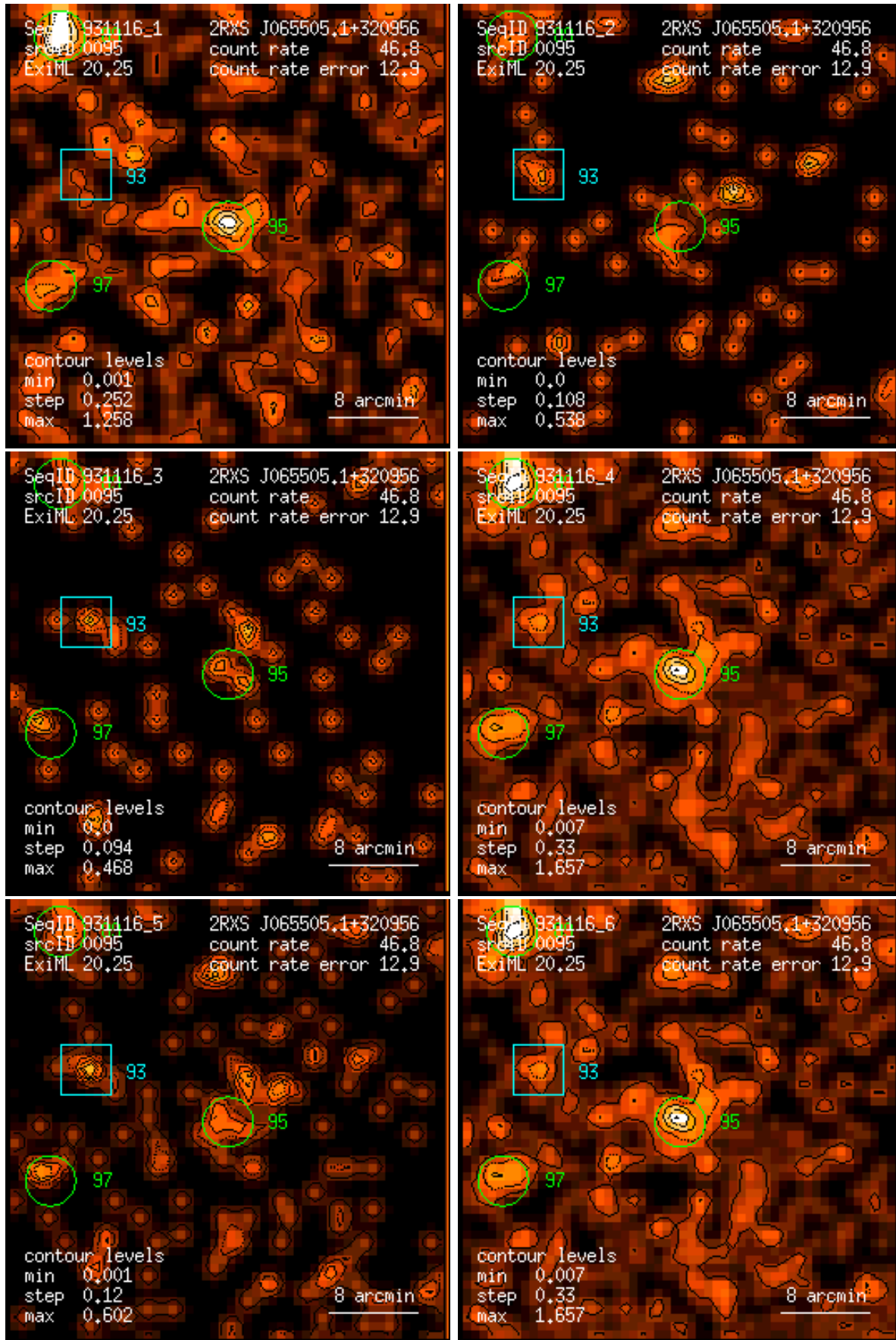
Figure 95: RASS 931116: detection 0095: band rate images, Gaussian filter: (1) PSPC channels 11 – 41, (2) 52 – 90, (3) 91 – 201, (4) 11 – 235, (5) 52 – 201, (6) 11 – 201. Broad band rates in counts/ks. Band rate contour levels in counts/ks/arcmin 2 .
