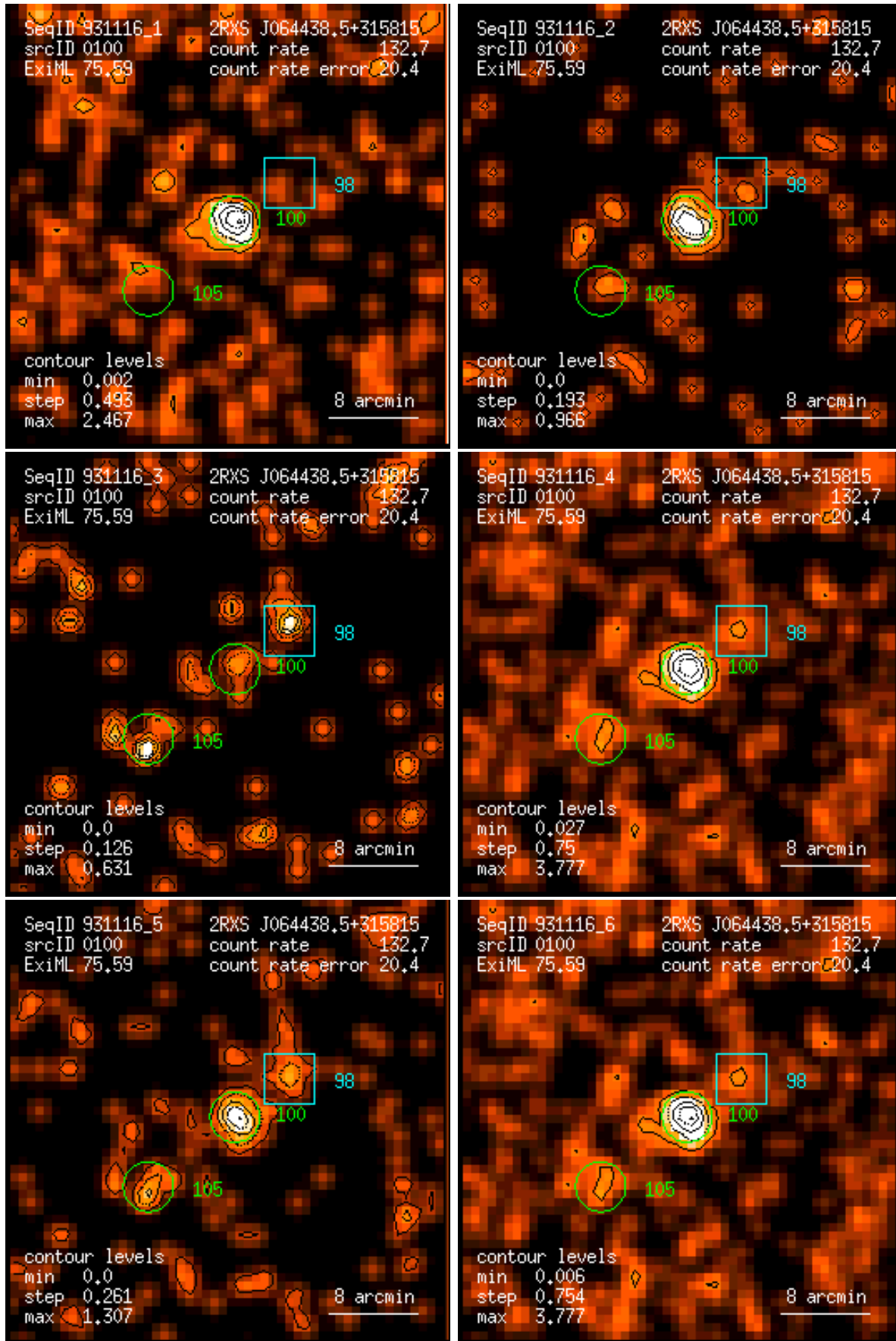
Figure 100: RASS 931116: detection 0100: band rate images, Gaussian filter: (1) PSPC channels 11 – 41, (2) 52 – 90, (3) 91 – 201, (4) 11 – 235, (5) 52 – 201, (6) 11 – 201. Broad band rates in counts/ks. Band rate contour levels in counts/ks/arcmin 2 .
