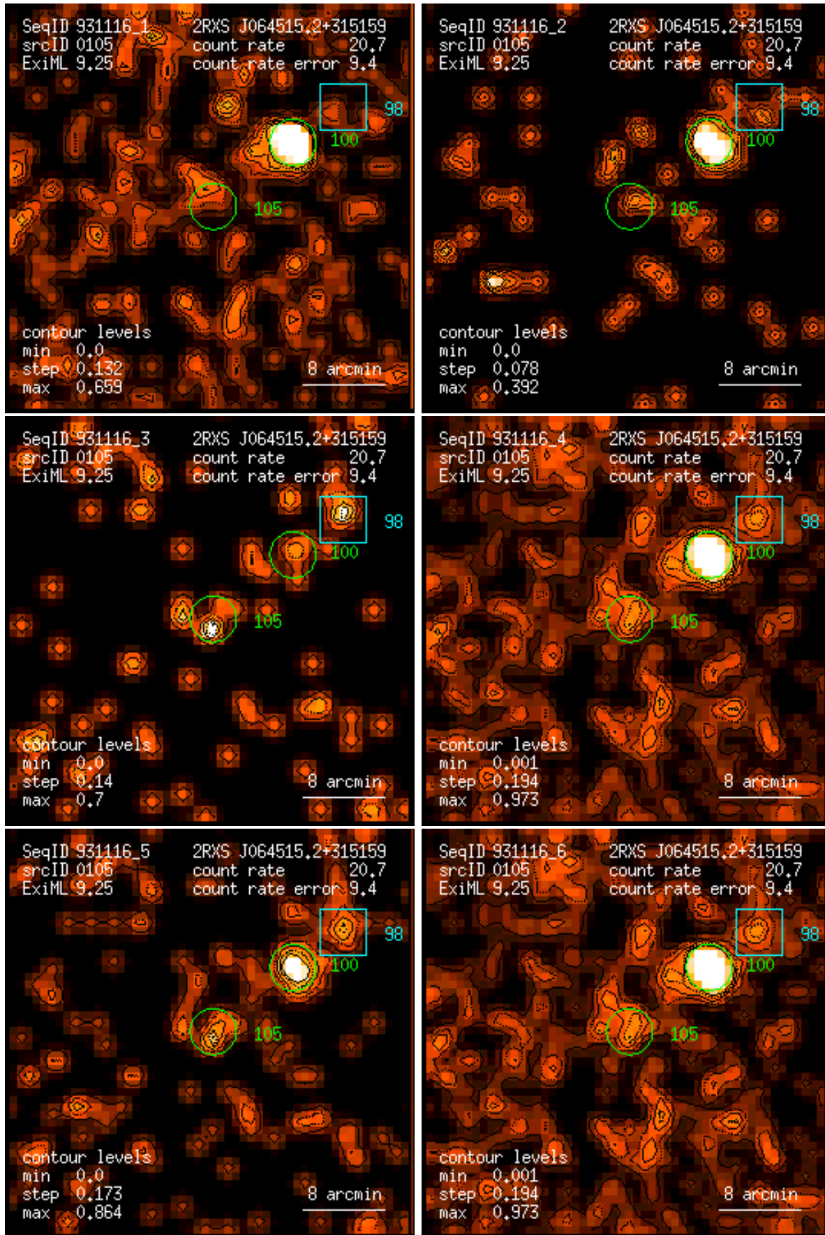
Figure 105: RASS 931116: detection 0105: band rate images, Gaussian filter: (1) PSPC channels 11 – 41, (2) 52 – 90, (3) 91 – 201, (4) 11 – 235, (5) 52 – 201, (6) 11 – 201. Broad band rates in counts/ks. Band rate contour levels in counts/ks/arcmin 2 .
