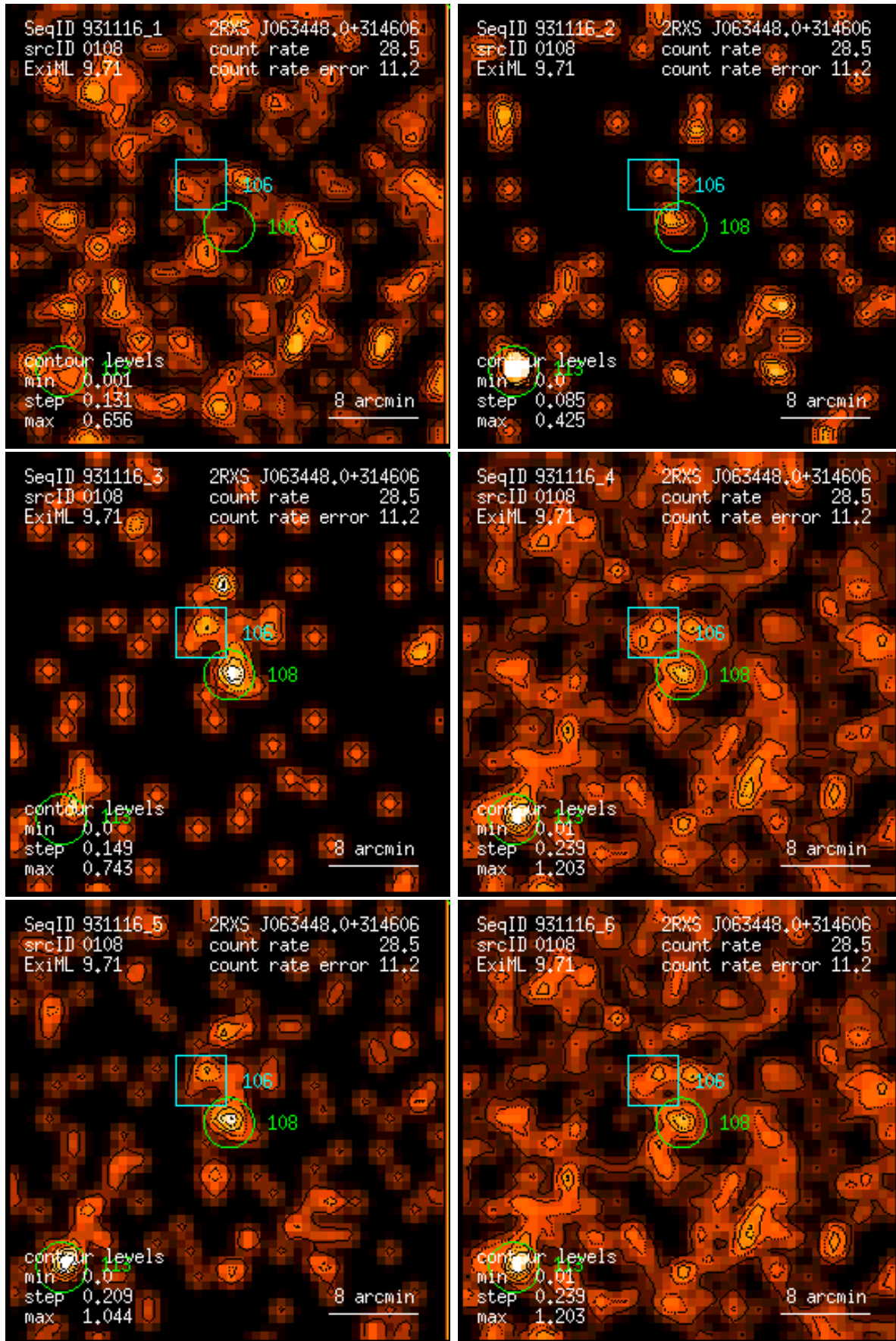
Figure 108: RASS 931116: detection 0108: band rate images, Gaussian filter: (1) PSPC channels 11 – 41, (2) 52 – 90, (3) 91 – 201, (4) 11 – 235, (5) 52 – 201, (6) 11 – 201. Broad band rates in counts/ks. Band rate contour levels in counts/ks/arcmin 2 .
