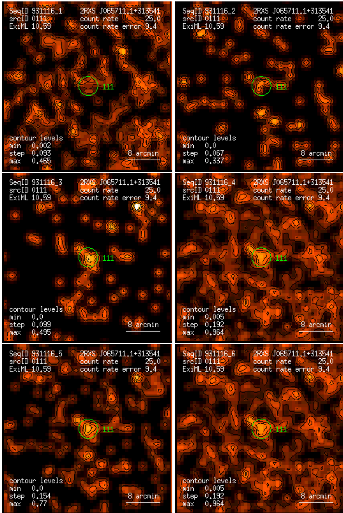
Figure 111: RASS 931116: detection 0111: band rate images, Gaussian filter: (1) PSPC channels 11 – 41, (2) 52 – 90, (3) 91 – 201, (4) 11 – 235, (5) 52 – 201, (6) 11 – 201. Broad band rates in counts/ks. Band rate contour levels in counts/ks/arcmin 2 .
