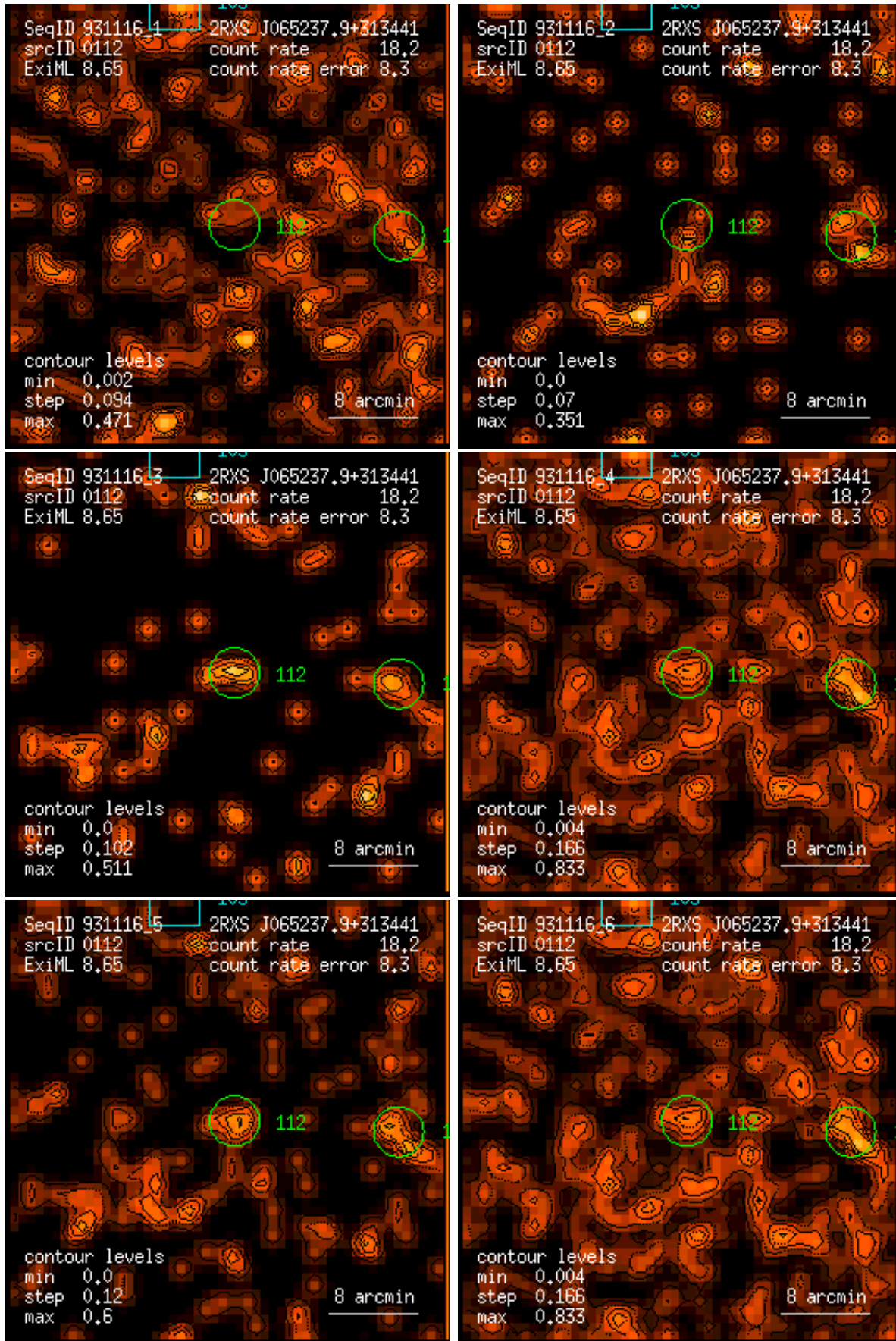
Figure 112: RASS 931116: detection 0112: band rate images, Gaussian filter: (1) PSPC channels 11 – 41, (2) 52 – 90, (3) 91 – 201, (4) 11 – 235, (5) 52 – 201, (6) 11 – 201. Broad band rates in counts/ks. Band rate contour levels in counts/ks/arcmin 2 .
