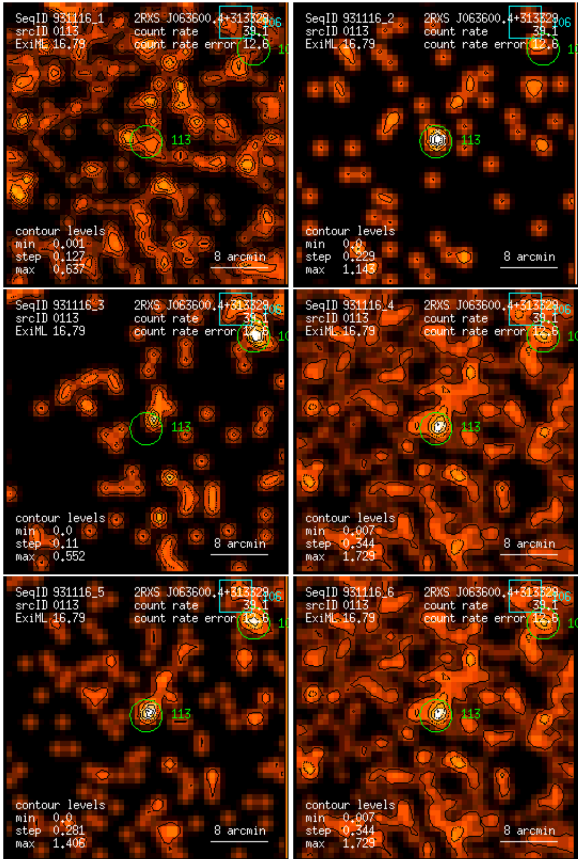
Figure 113: RASS 931116: detection 0113: band rate images, Gaussian filter: (1) PSPC channels 11 – 41, (2) 52 – 90, (3) 91 – 201, (4) 11 – 235, (5) 52 – 201, (6) 11 – 201. Broad band rates in counts/ks. Band rate contour levels in counts/ks/arcmin 2 .
