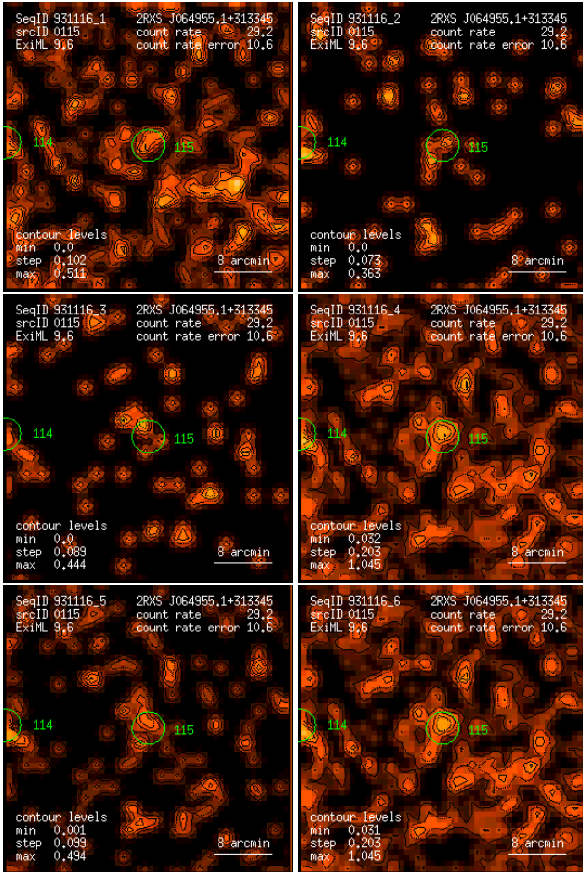
Figure 115: RASS 931116: detection 0115: band rate images, Gaussian filter: (1) PSPC channels 11 – 41, (2) 52 – 90, (3) 91 – 201, (4) 11 – 235, (5) 52 – 201, (6) 11 – 201. Broad band rates in counts/ks. Band rate contour levels in counts/ks/arcmin 2 .
