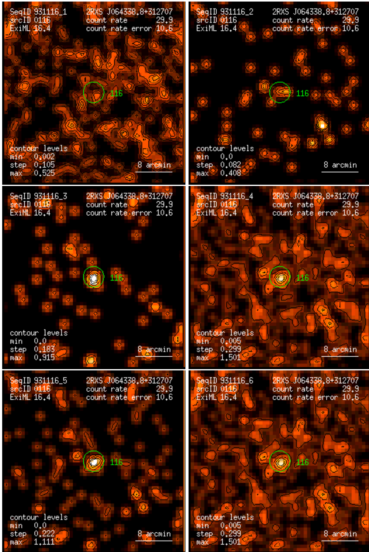
Figure 116: RASS 931116: detection 0116: band rate images, Gaussian filter: (1) PSPC channels 11 – 41, (2) 52 – 90, (3) 91 – 201, (4) 11 – 235, (5) 52 – 201, (6) 11 – 201. Broad band rates in counts/ks. Band rate contour levels in counts/ks/arcmin 2 .
