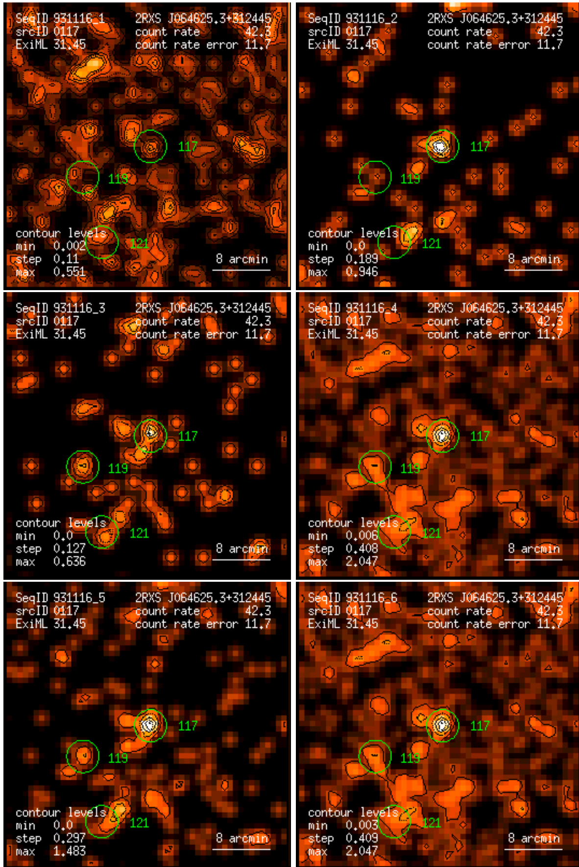
Figure 117: RASS 931116: detection 0117: band rate images, Gaussian filter: (1) PSPC channels 11 – 41, (2) 52 – 90, (3) 91 – 201, (4) 11 – 235, (5) 52 – 201, (6) 11 – 201. Broad band rates in counts/ks. Band rate contour levels in counts/ks/arcmin 2 .
