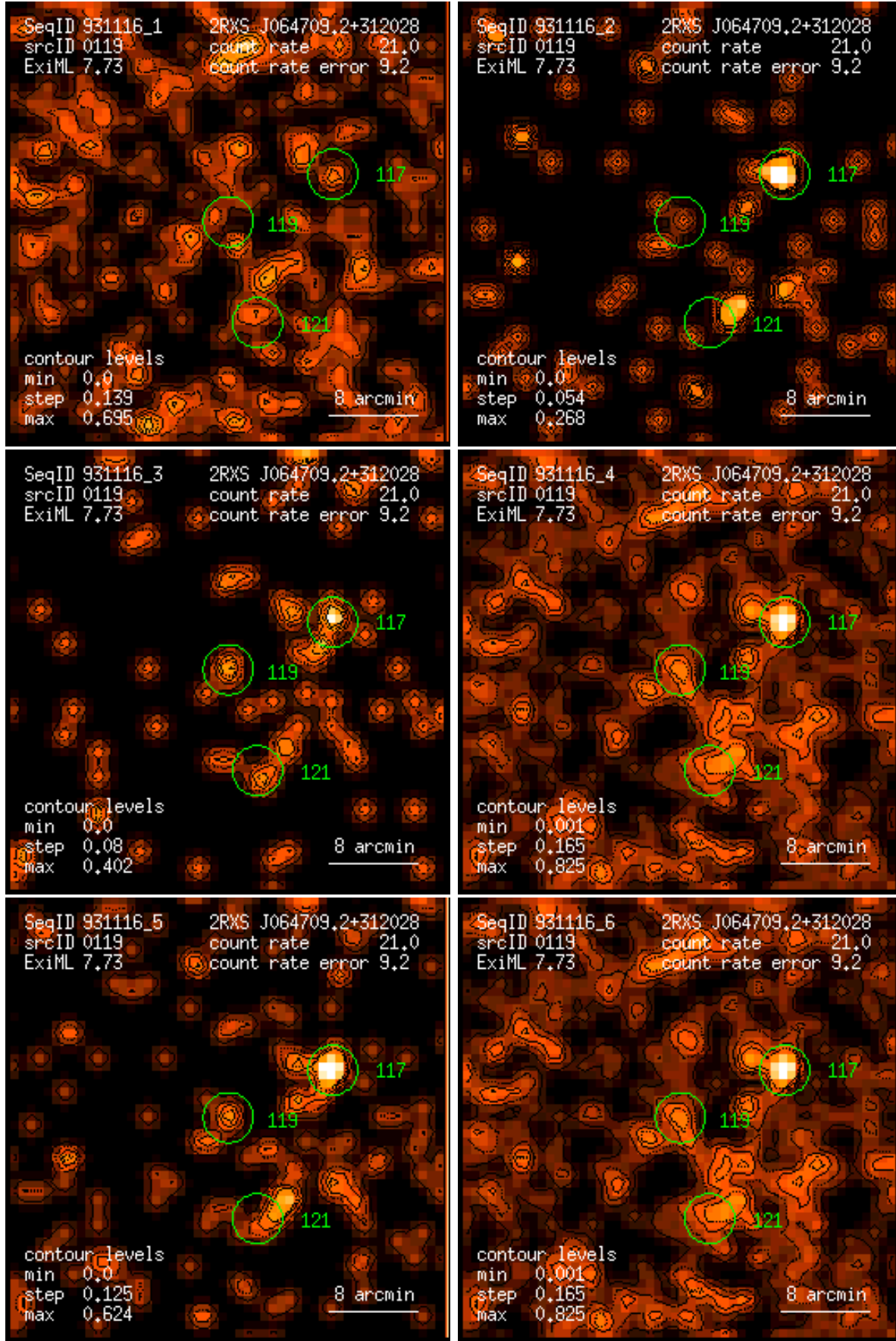
Figure 119: RASS 931116: detection 0119: band rate images, Gaussian filter: (1) PSPC channels 11 – 41, (2) 52 – 90, (3) 91 – 201, (4) 11 – 235, (5) 52 – 201, (6) 11 – 201. Broad band rates in counts/ks. Band rate contour levels in counts/ks/arcmin 2 .
