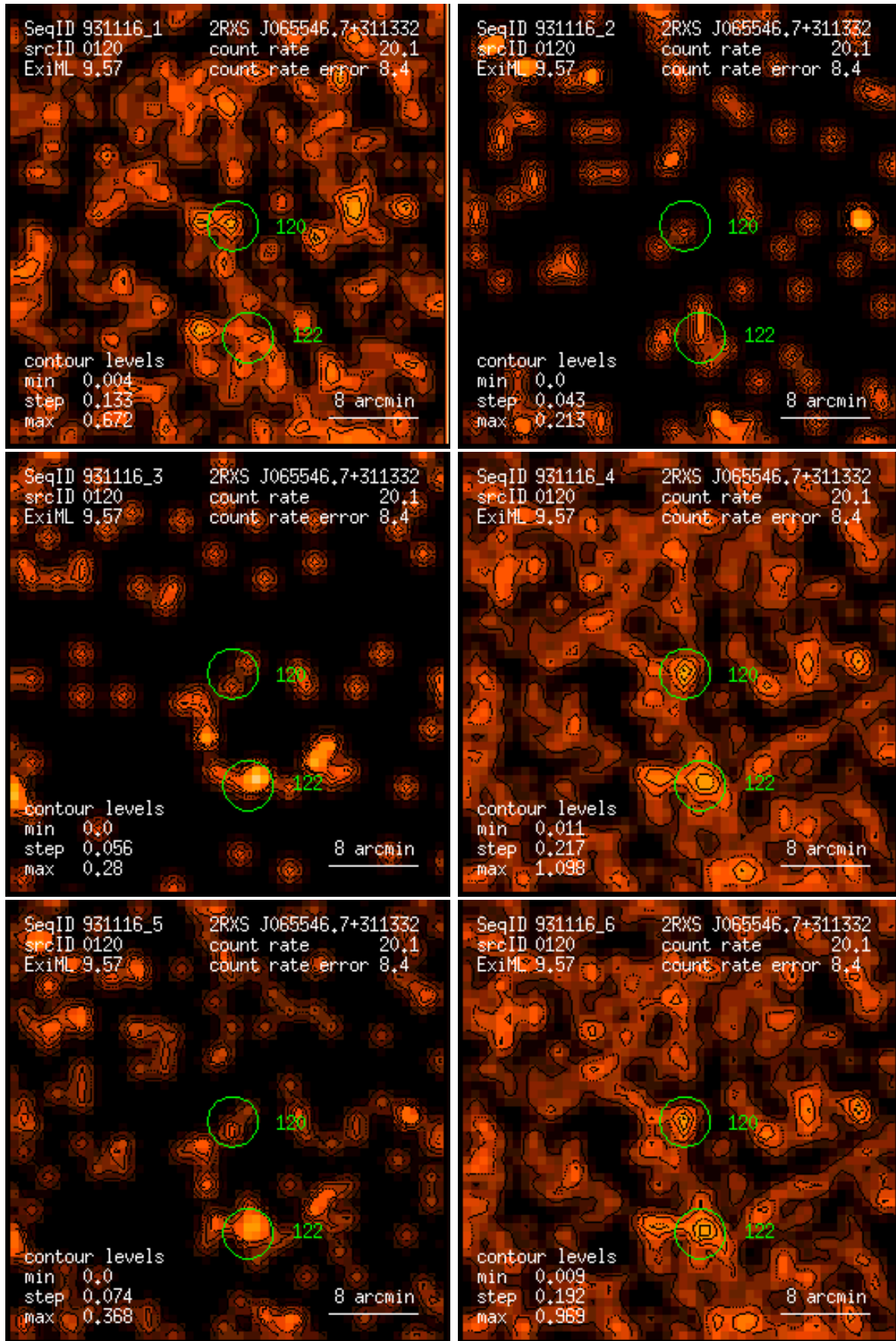
Figure 120: RASS 931116: detection 0120: band rate images, Gaussian filter: (1) PSPC channels 11 – 41, (2) 52 – 90, (3) 91 – 201, (4) 11 – 235, (5) 52 – 201, (6) 11 – 201. Broad band rates in counts/ks. Band rate contour levels in counts/ks/arcmin 2 .
