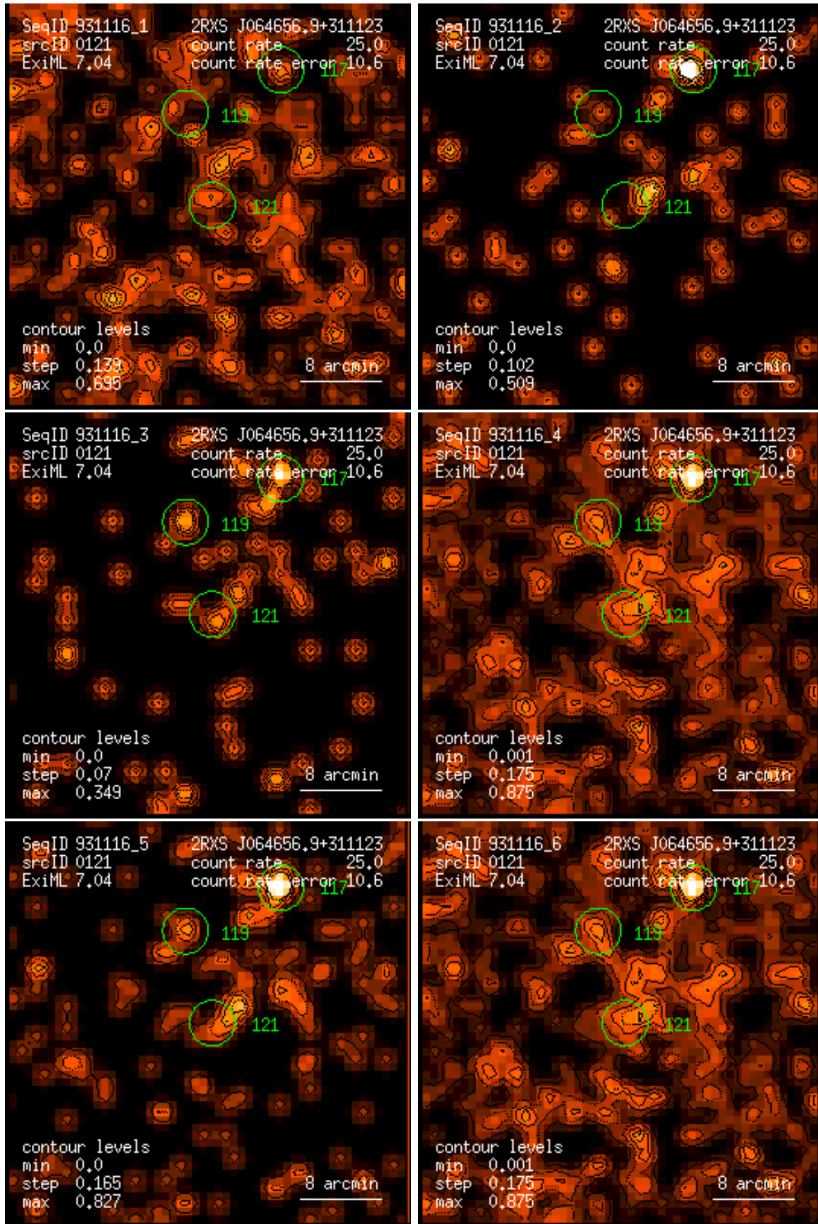
Figure 121: RASS 931116: detection 0121: band rate images, Gaussian filter: (1) PSPC channels 11 – 41, (2) 52 – 90, (3) 91 – 201, (4) 11 – 235, (5) 52 – 201, (6) 11 – 201. Broad band rates in counts/ks. Band rate contour levels in counts/ks/arcmin 2 .
