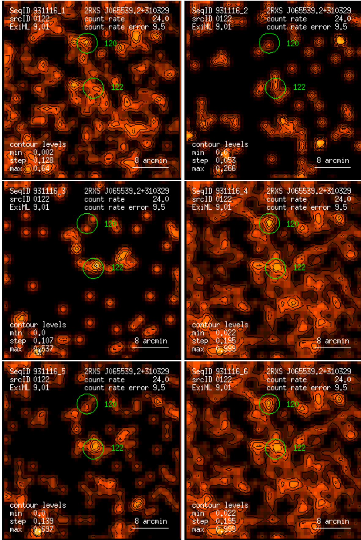
Figure 122: RASS 931116: detection 0122: band rate images, Gaussian filter: (1) PSPC channels 11 – 41, (2) 52 – 90, (3) 91 – 201, (4) 11 – 235, (5) 52 – 201, (6) 11 – 201. Broad band rates in counts/ks. Band rate contour levels in counts/ks/arcmin 2 .
