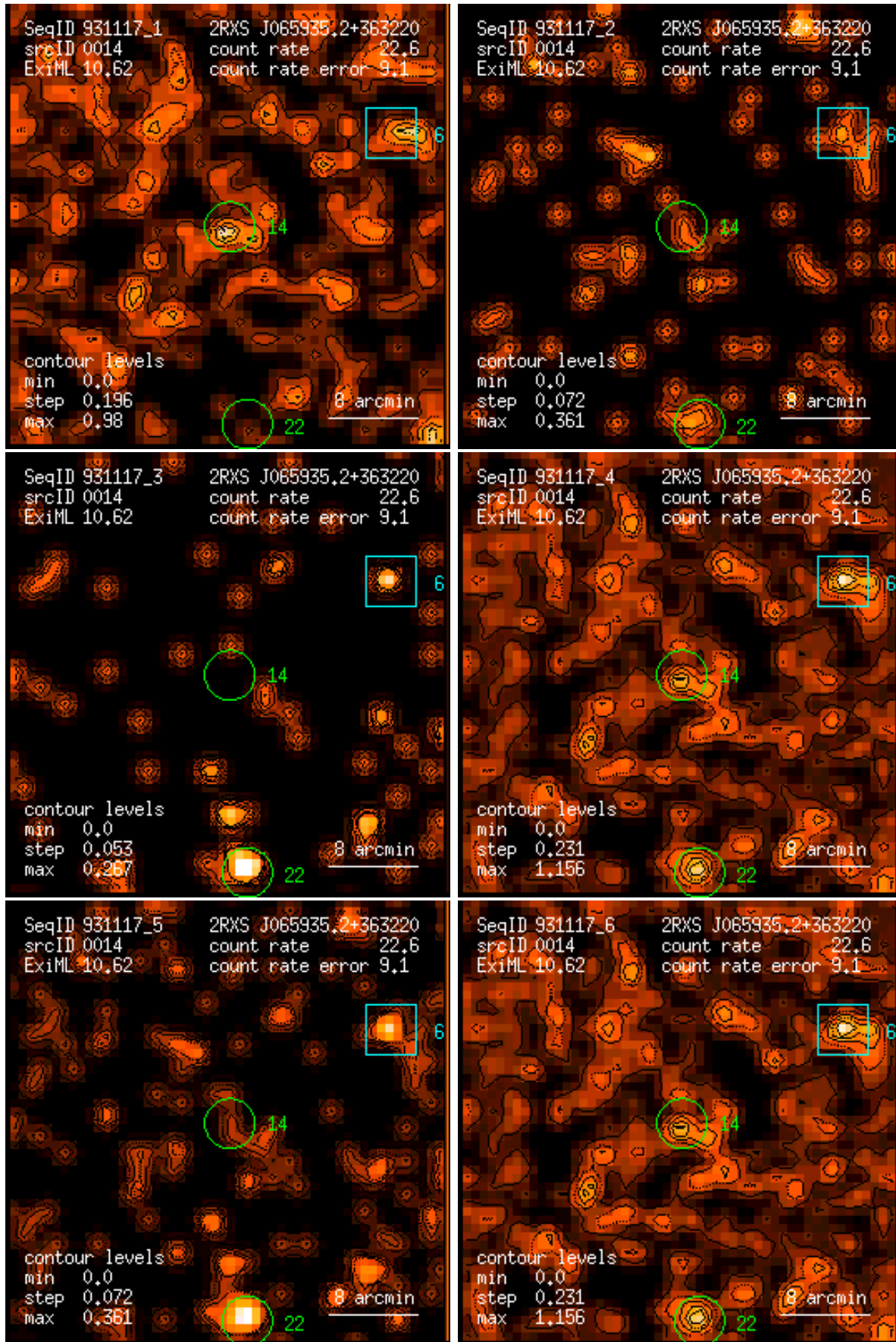
Figure 14: RASS 931117: detection 0014: band rate images, Gaussian filter: (1) PSPC channels 11 – 41, (2) 52 – 90, (3) 91 – 201, (4) 11 – 235, (5) 52 – 201, (6) 11 – 201. Broad band rates in counts/ks. Band rate contour levels in counts/ks/arcmin 2 .
