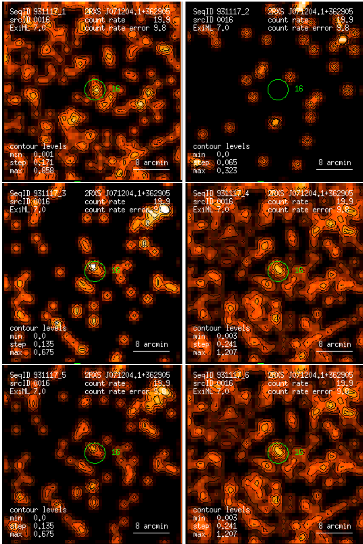
Figure 16: RASS 931117: detection 0016: band rate images, Gaussian filter: (1) PSPC channels 11 – 41, (2) 52 – 90, (3) 91 – 201, (4) 11 – 235, (5) 52 – 201, (6) 11 – 201. Broad band rates in counts/ks. Band rate contour levels in counts/ks/arcmin 2 .
