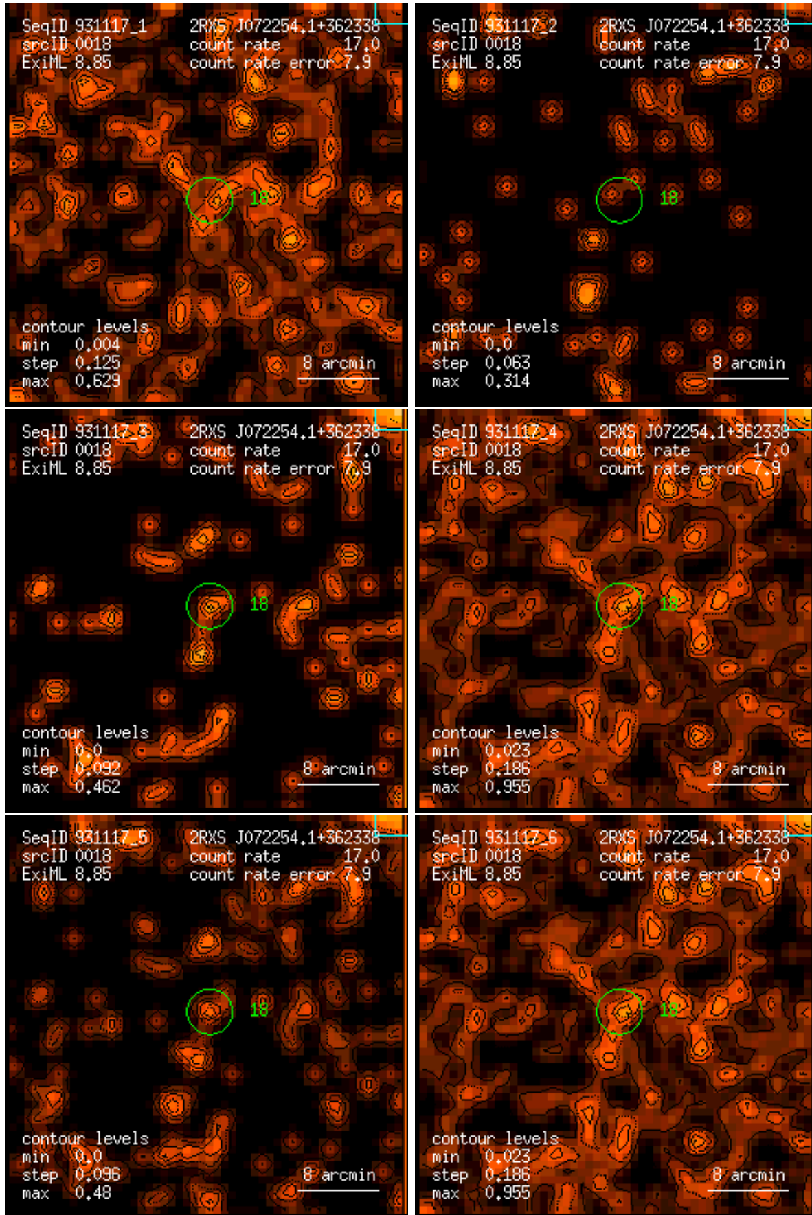
Figure 18: RASS 931117: detection 0018: band rate images, Gaussian filter: (1) PSPC channels 11 – 41, (2) 52 – 90, (3) 91 – 201, (4) 11 – 235, (5) 52 – 201, (6) 11 – 201. Broad band rates in counts/ks. Band rate contour levels in counts/ks/arcmin 2 .
