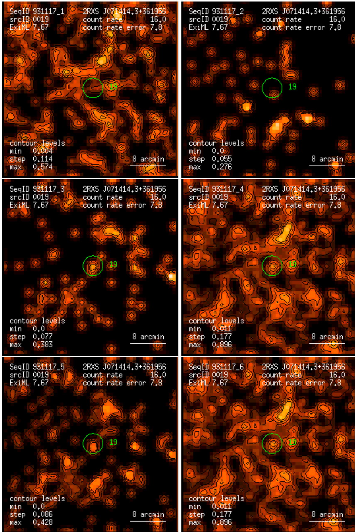
Figure 19: RASS 931117: detection 0019: band rate images, Gaussian filter: (1) PSPC channels 11 – 41, (2) 52 – 90, (3) 91 – 201, (4) 11 – 235, (5) 52 – 201, (6) 11 – 201. Broad band rates in counts/ks. Band rate contour levels in counts/ks/arcmin 2 .
