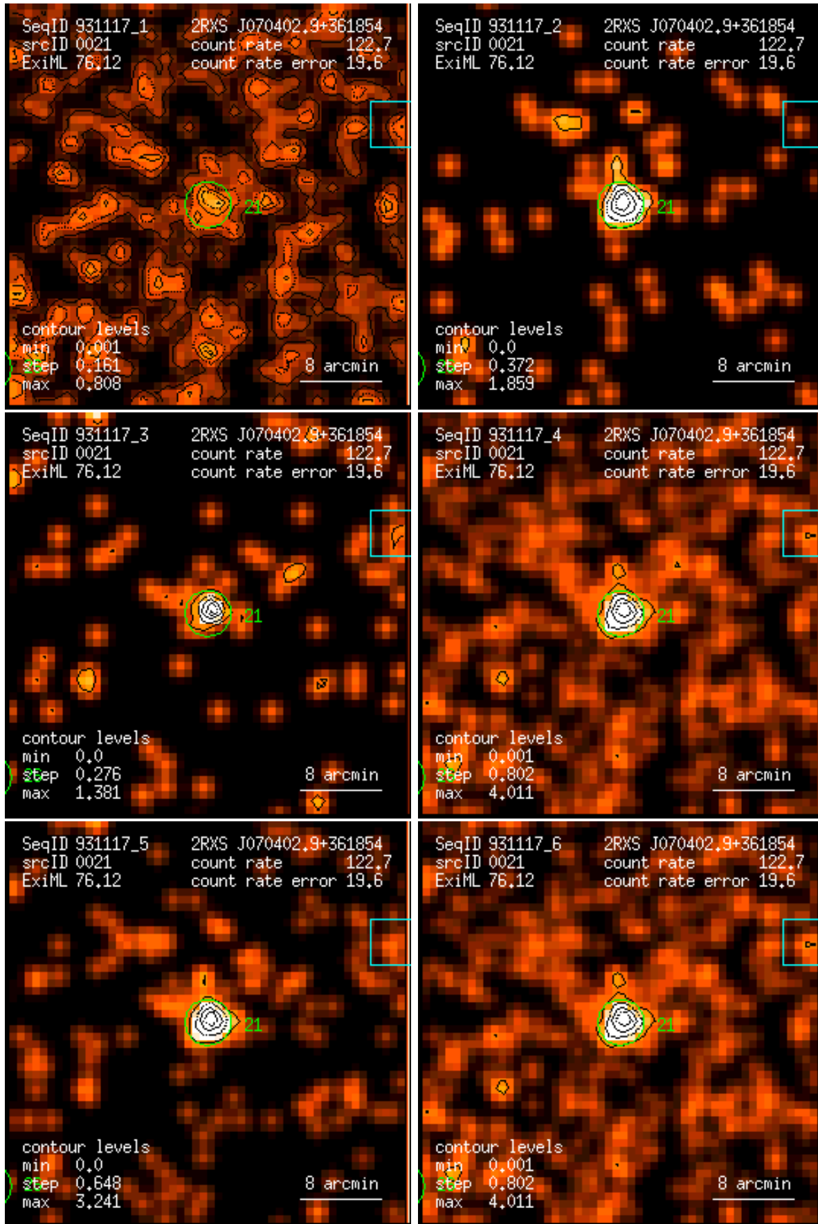
Figure 21: RASS 931117: detection 0021: band rate images, Gaussian filter: (1) PSPC channels 11 – 41, (2) 52 – 90, (3) 91 – 201, (4) 11 – 235, (5) 52 – 201, (6) 11 – 201. Broad band rates in counts/ks. Band rate contour levels in counts/ks/arcmin 2 .
