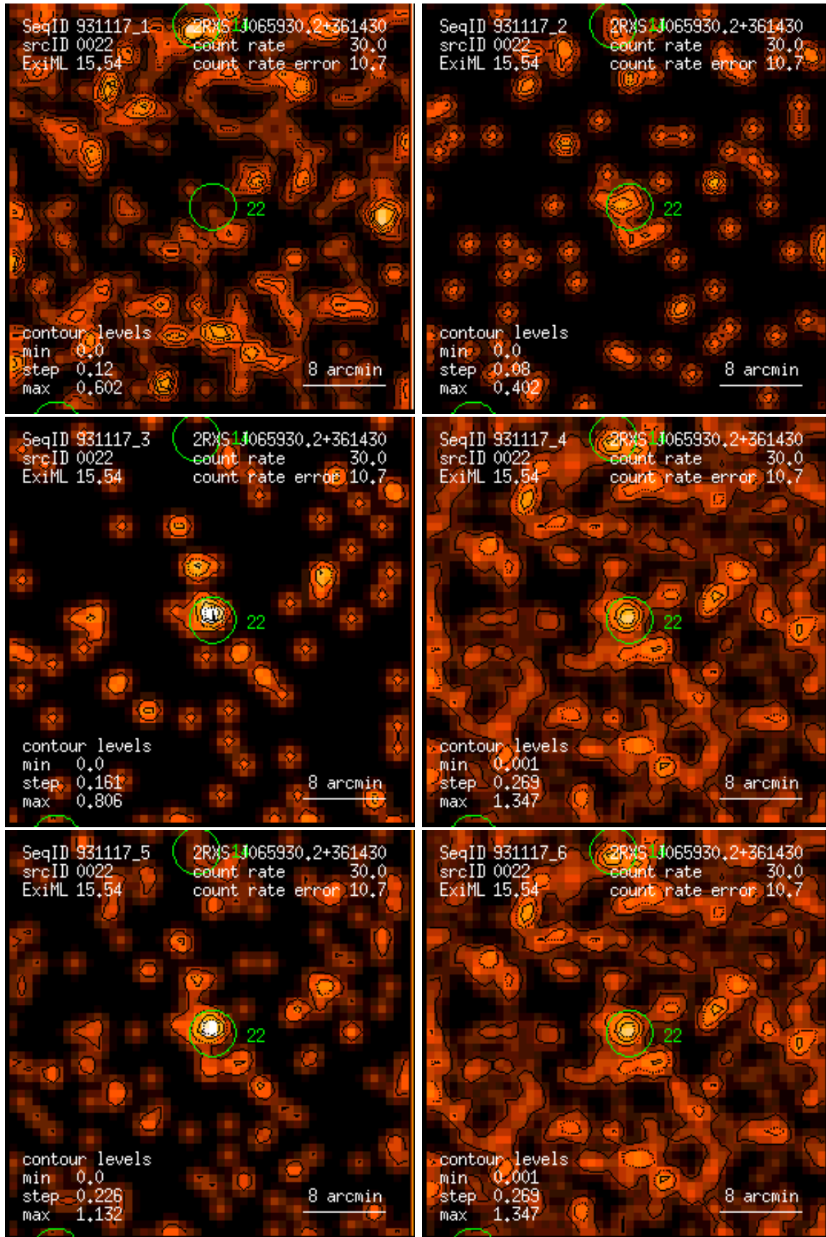
Figure 22: RASS 931117: detection 0022: band rate images, Gaussian filter: (1) PSPC channels 11 – 41, (2) 52 – 90, (3) 91 – 201, (4) 11 – 235, (5) 52 – 201, (6) 11 – 201. Broad band rates in counts/ks. Band rate contour levels in counts/ks/arcmin 2 .
