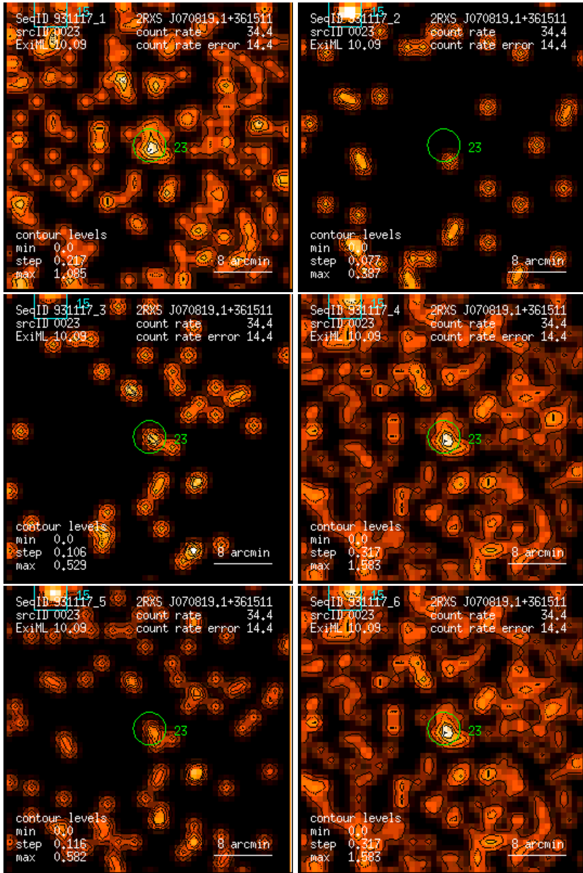
Figure 23: RASS 931117: detection 0023: band rate images, Gaussian filter: (1) PSPC channels 11 – 41, (2) 52 – 90, (3) 91 – 201, (4) 11 – 235, (5) 52 – 201, (6) 11 – 201. Broad band rates in counts/ks. Band rate contour levels in counts/ks/arcmin 2 .
