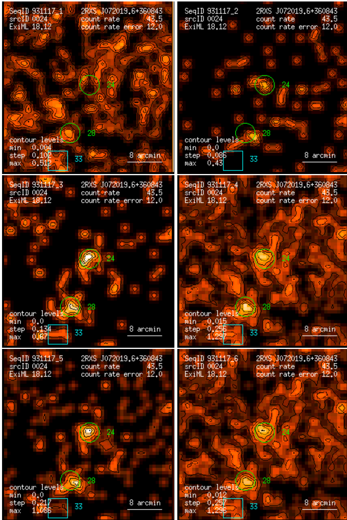
Figure 24: RASS 931117: detection 0024: band rate images, Gaussian filter: (1) PSPC channels 11 – 41, (2) 52 – 90, (3) 91 – 201, (4) 11 – 235, (5) 52 – 201, (6) 11 – 201. Broad band rates in counts/ks. Band rate contour levels in counts/ks/arcmin 2 .
