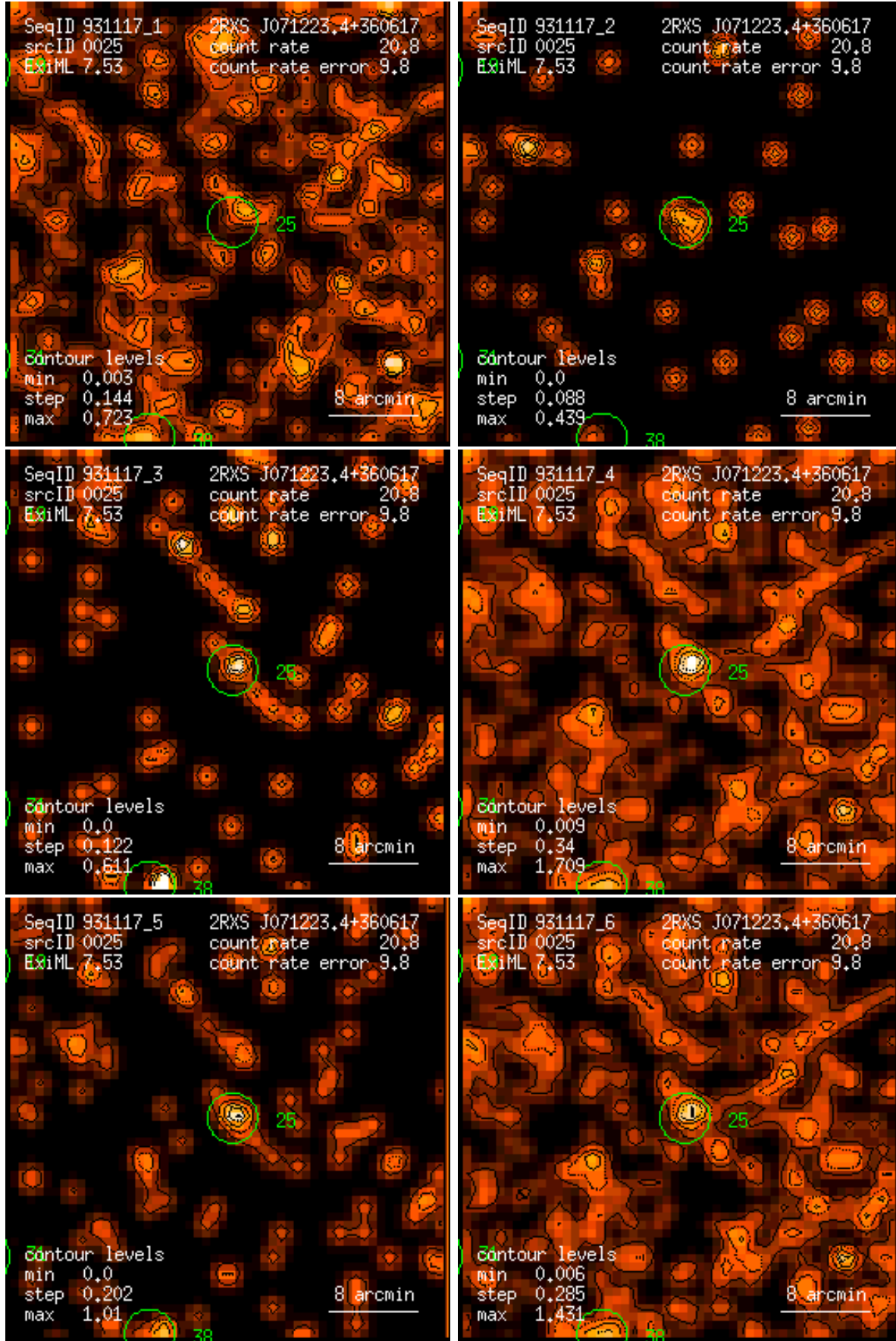
Figure 25: RASS 931117: detection 0025: band rate images, Gaussian filter: (1) PSPC channels 11 – 41, (2) 52 – 90, (3) 91 – 201, (4) 11 – 235, (5) 52 – 201, (6) 11 – 201. Broad band rates in counts/ks. Band rate contour levels in counts/ks/arcmin 2 .
