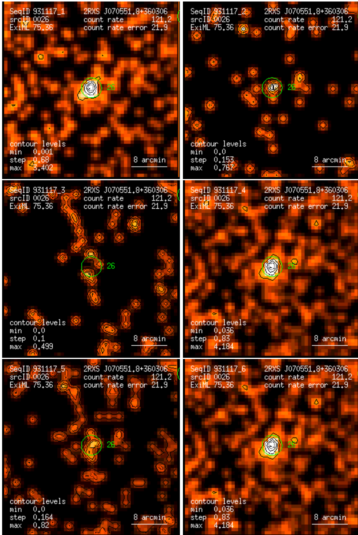
Figure 26: RASS 931117: detection 0026: band rate images, Gaussian filter: (1) PSPC channels 11 – 41, (2) 52 – 90, (3) 91 – 201, (4) 11 – 235, (5) 52 – 201, (6) 11 – 201. Broad band rates in counts/ks. Band rate contour levels in counts/ks/arcmin 2 .
