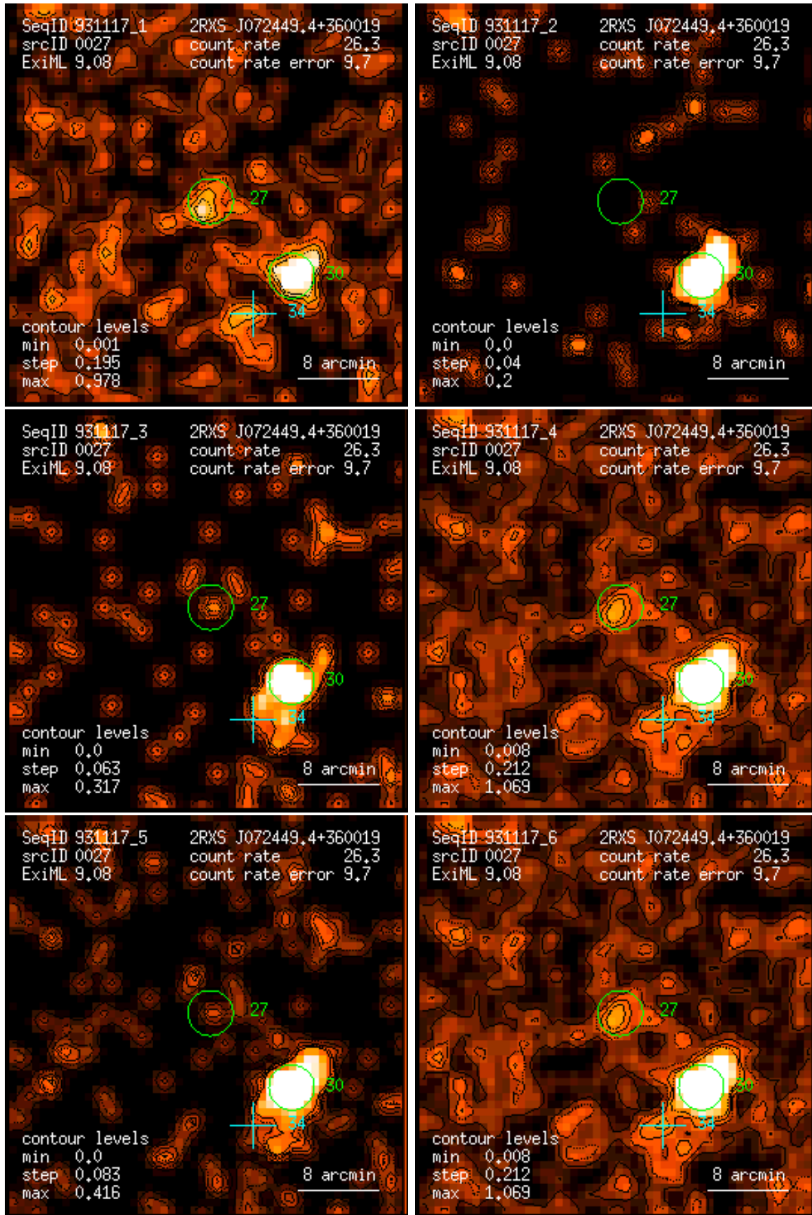
Figure 27: RASS 931117: detection 0027: band rate images, Gaussian filter: (1) PSPC channels 11 – 41, (2) 52 – 90, (3) 91 – 201, (4) 11 – 235, (5) 52 – 201, (6) 11 – 201. Broad band rates in counts/ks. Band rate contour levels in counts/ks/arcmin 2 .
