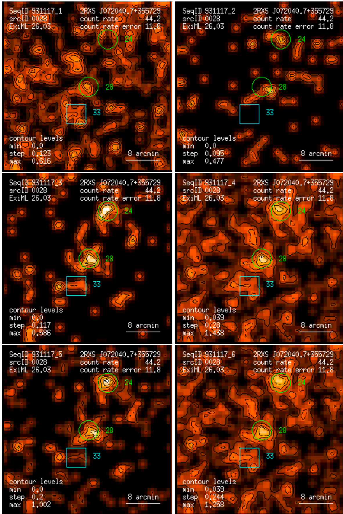
Figure 28: RASS 931117: detection 0028: band rate images, Gaussian filter: (1) PSPC channels 11 – 41, (2) 52 – 90, (3) 91 – 201, (4) 11 – 235, (5) 52 – 201, (6) 11 – 201. Broad band rates in counts/ks. Band rate contour levels in counts/ks/arcmin 2 .
