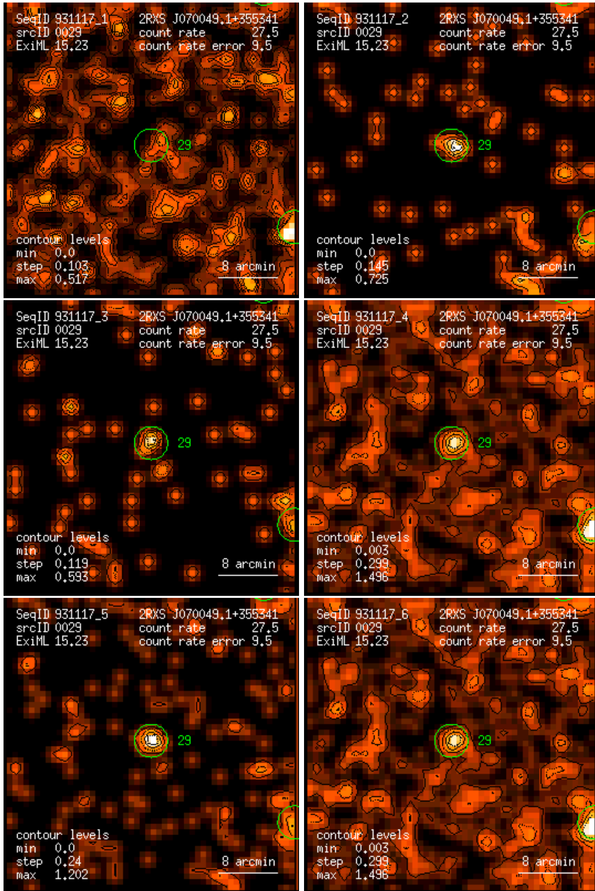
Figure 29: RASS 931117: detection 0029: band rate images, Gaussian filter: (1) PSPC channels 11 – 41, (2) 52 – 90, (3) 91 – 201, (4) 11 – 235, (5) 52 – 201, (6) 11 – 201. Broad band rates in counts/ks. Band rate contour levels in counts/ks/arcmin 2 .
