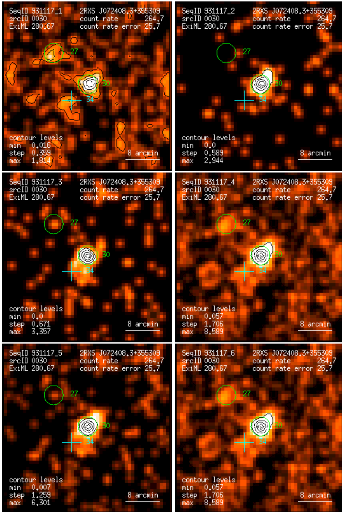
Figure 30: RASS 931117: detection 0030: band rate images, Gaussian filter: (1) PSPC channels 11 – 41, (2) 52 – 90, (3) 91 – 201, (4) 11 – 235, (5) 52 – 201, (6) 11 – 201. Broad band rates in counts/ks. Band rate contour levels in counts/ks/arcmin 2 .
