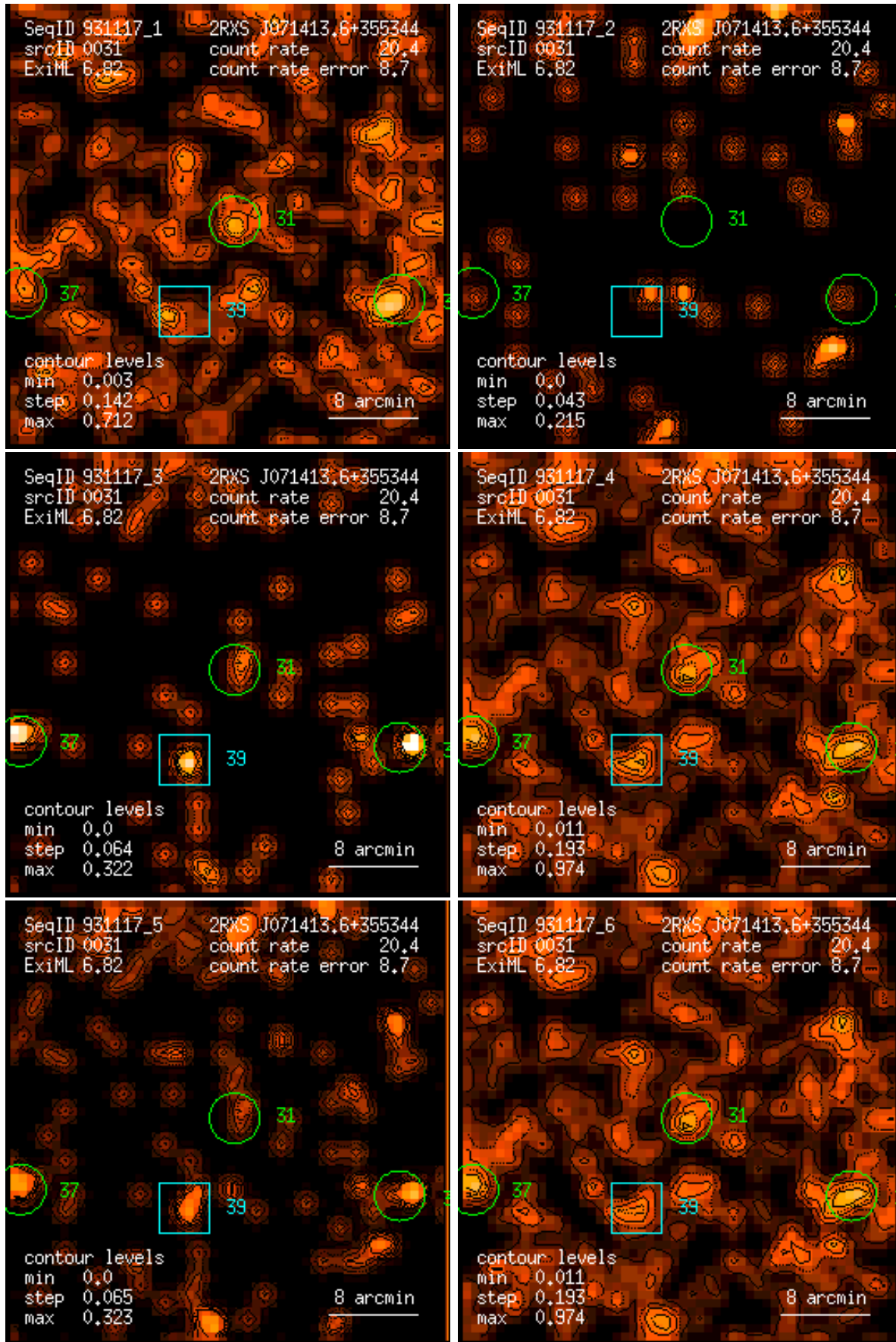
Figure 31: RASS 931117: detection 0031: band rate images, Gaussian filter: (1) PSPC channels 11 – 41, (2) 52 – 90, (3) 91 – 201, (4) 11 – 235, (5) 52 – 201, (6) 11 – 201. Broad band rates in counts/ks. Band rate contour levels in counts/ks/arcmin 2 .
