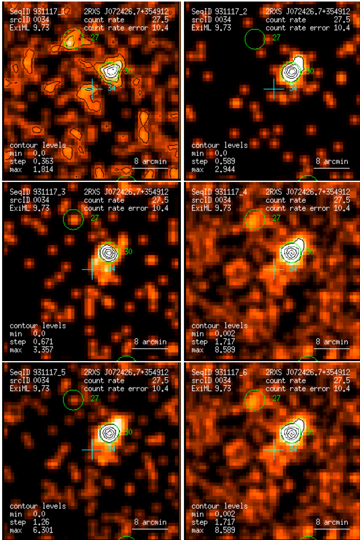
Figure 34: RASS 931117: detection 0034: band rate images, Gaussian filter: (1) PSPC channels 11 – 41, (2) 52 – 90, (3) 91 – 201, (4) 11 – 235, (5) 52 – 201, (6) 11 – 201. Broad band rates in counts/ks. Band rate contour levels in counts/ks/arcmin 2 .
