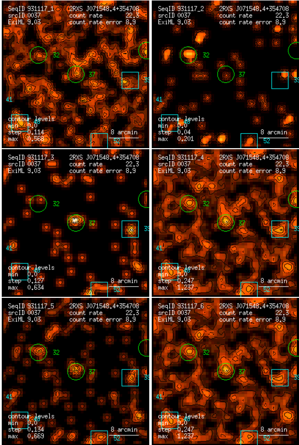
Figure 37: RASS 931117: detection 0037: band rate images, Gaussian filter: (1) PSPC channels 11 – 41, (2) 52 – 90, (3) 91 – 201, (4) 11 – 235, (5) 52 – 201, (6) 11 – 201. Broad band rates in counts/ks. Band rate contour levels in counts/ks/arcmin 2 .
