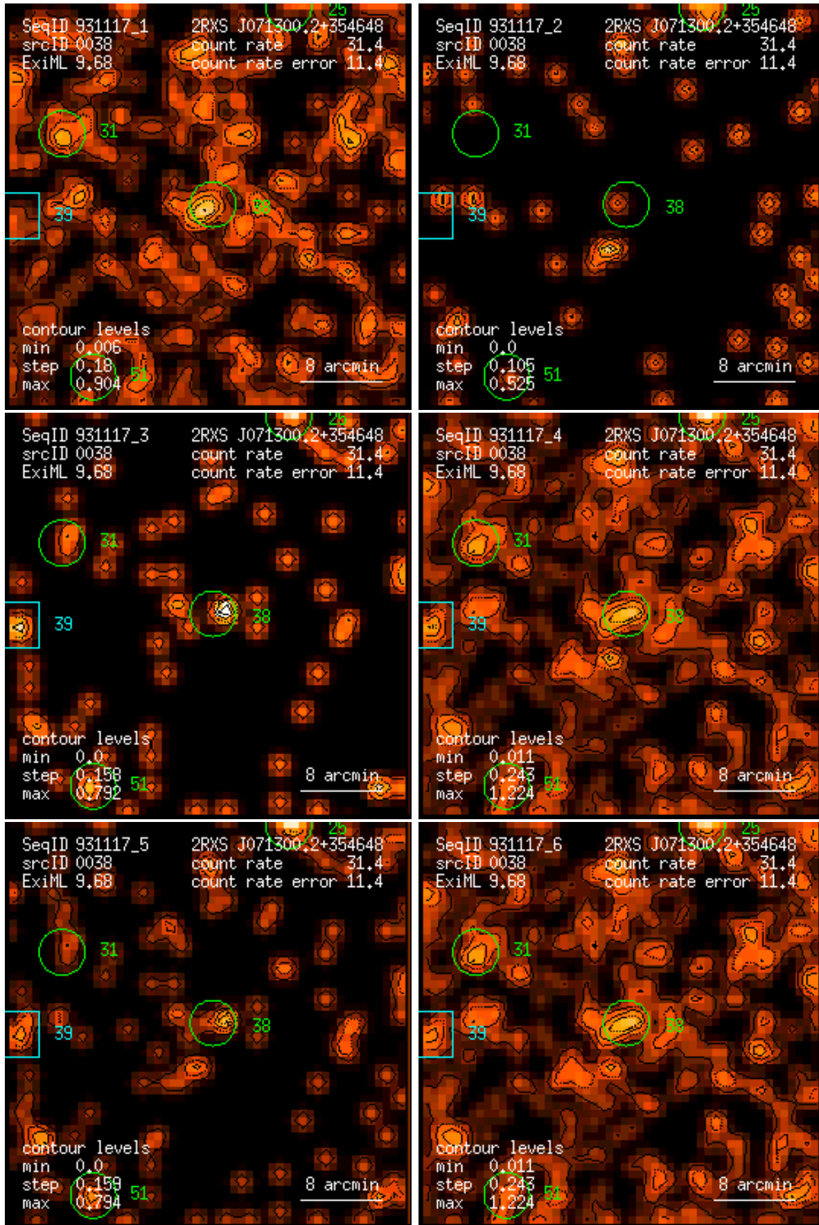
Figure 38: RASS 931117: detection 0038: band rate images, Gaussian filter: (1) PSPC channels 11 – 41, (2) 52 – 90, (3) 91 – 201, (4) 11 – 235, (5) 52 – 201, (6) 11 – 201. Broad band rates in counts/ks. Band rate contour levels in counts/ks/arcmin 2 .
