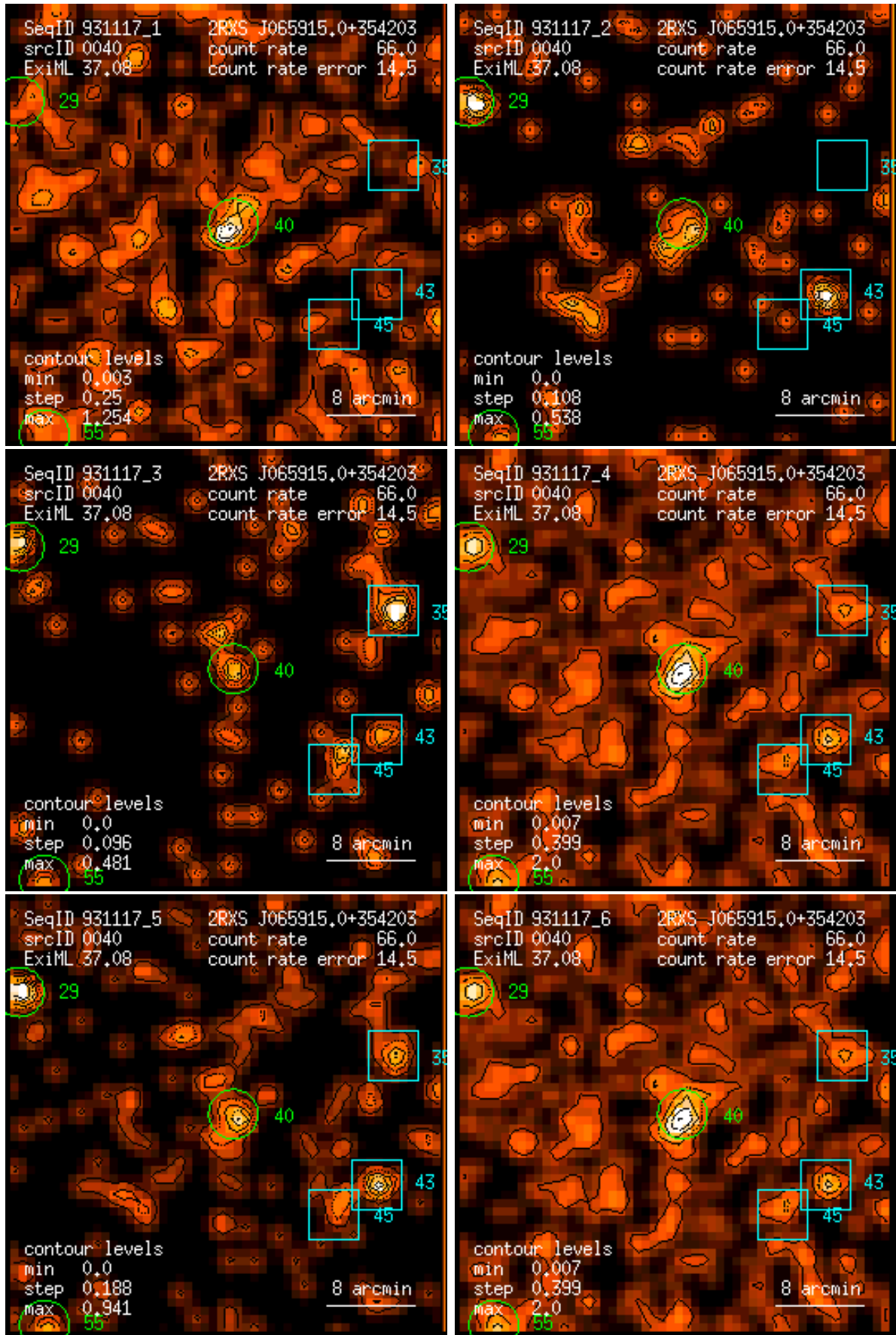
Figure 40: RASS 931117: detection 0040: band rate images, Gaussian filter: (1) PSPC channels 11 – 41, (2) 52 – 90, (3) 91 – 201, (4) 11 – 235, (5) 52 – 201, (6) 11 – 201. Broad band rates in counts/ks. Band rate contour levels in counts/ks/arcmin 2 .
