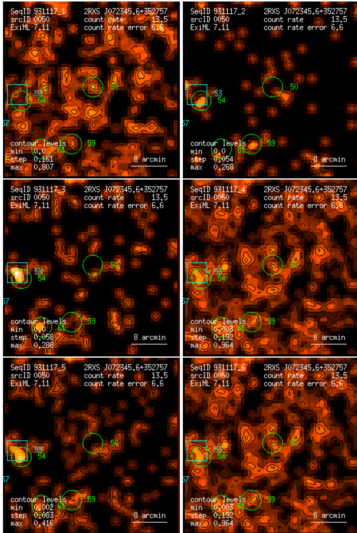
Figure 50: RASS 931117: detection 0050: band rate images, Gaussian filter: (1) PSPC channels 11 – 41, (2) 52 – 90, (3) 91 – 201, (4) 11 – 235, (5) 52 – 201, (6) 11 – 201. Broad band rates in counts/ks. Band rate contour levels in counts/ks/arcmin 2 .
