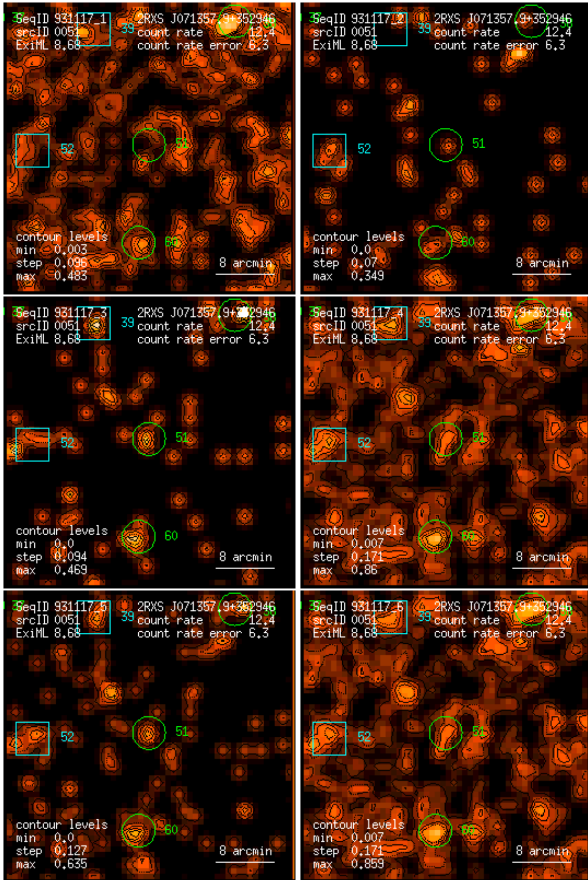
Figure 51: RASS 931117: detection 0051: band rate images, Gaussian filter: (1) PSPC channels 11 – 41, (2) 52 – 90, (3) 91 – 201, (4) 11 – 235, (5) 52 – 201, (6) 11 – 201. Broad band rates in counts/ks. Band rate contour levels in counts/ks/arcmin 2 .
