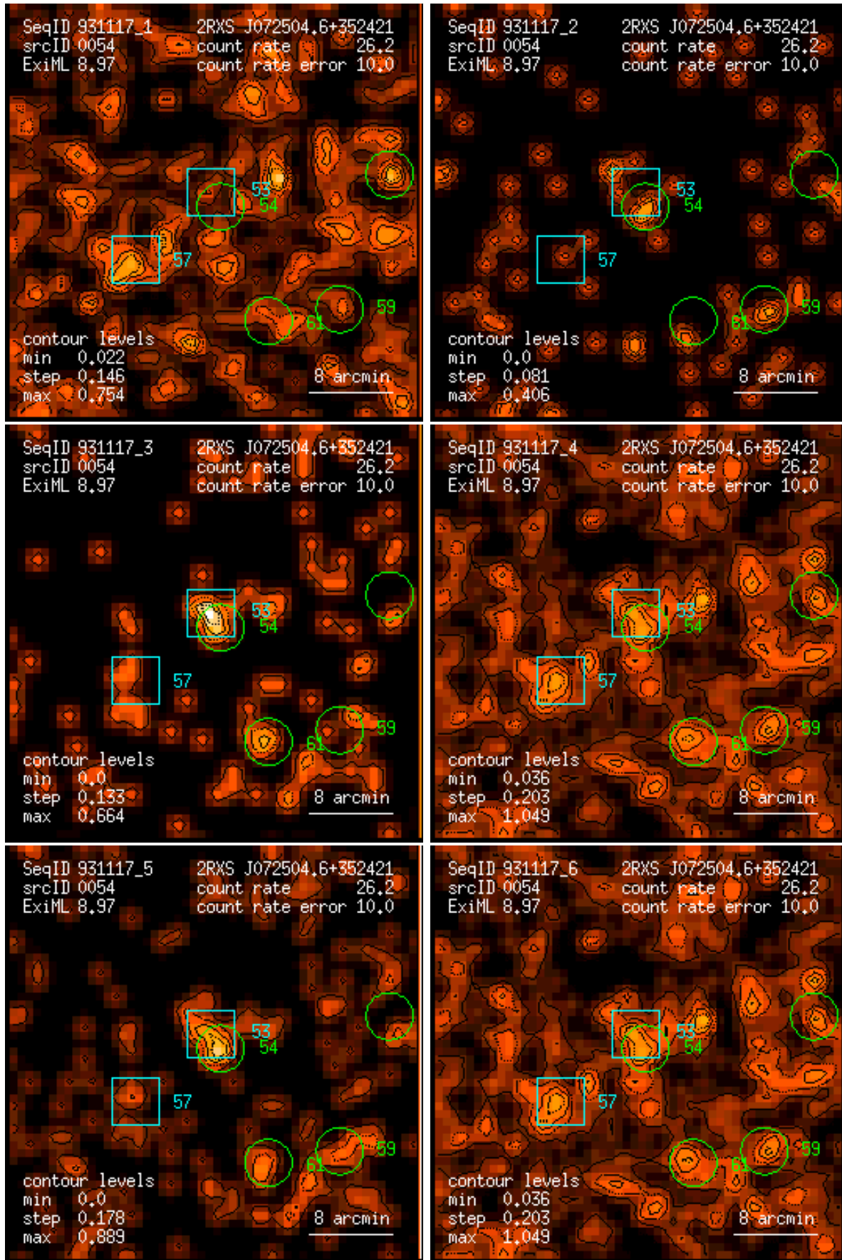
Figure 54: RASS 931117: detection 0054: band rate images, Gaussian filter: (1) PSPC channels 11 – 41, (2) 52 – 90, (3) 91 – 201, (4) 11 – 235, (5) 52 – 201, (6) 11 – 201. Broad band rates in counts/ks. Band rate contour levels in counts/ks/arcmin 2 .
